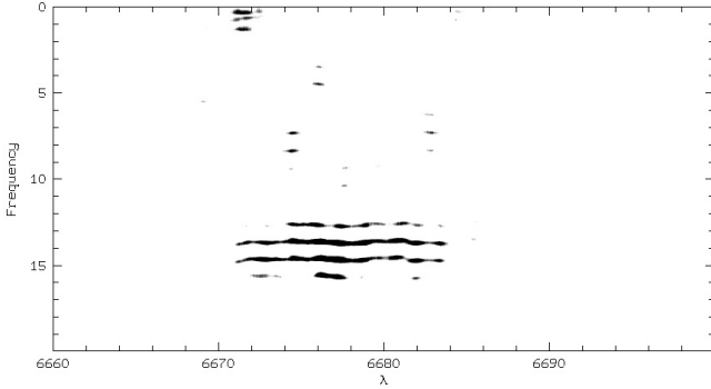
Fig. 5. Grey-scale 2D Fourier power spectrum of the He I \lambda 6678 line as derived from the April 2005 data.
