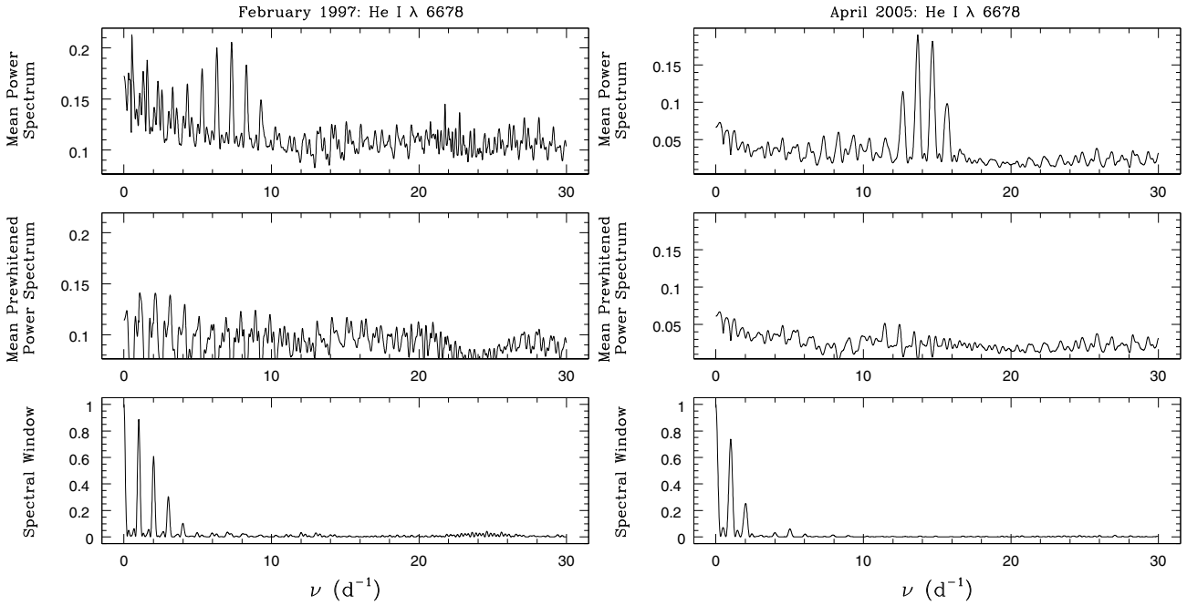
Fig. 4. Left: the top panel yields the mean Fourier power spectrum of the February 1997 He I \lambda 6678 data as derived from the 2D Fourier spectrum averaged over the profile of the He I \lambda 6678 line (from 6660 to 6700 Å). The middle panel indicates the mean power spectrum prewhitened for the two dominant frequencies (0.54 and 7.30 d -1 ) simultaneously. The lower panel yields the power spectral window resulting from the sampling of the February 1997 time series. Right: same for the April 2005 data. The frequencies used for the prewhitening are \nu_1 = 13.68 and \nu_2 = 8.31 d -1 in this case.
