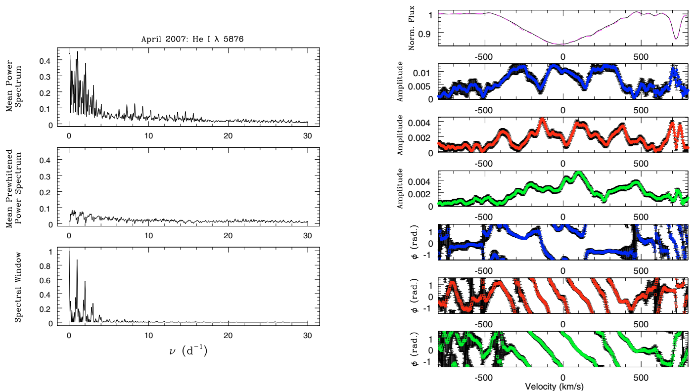
Fig. 9. Same as Fig. 8 but for the He I \lambda 5876 line as observed in April 2007. The frequencies used for prewhitening are 1.06, 14.62 and 8.25 \text{d}^{-1} .
