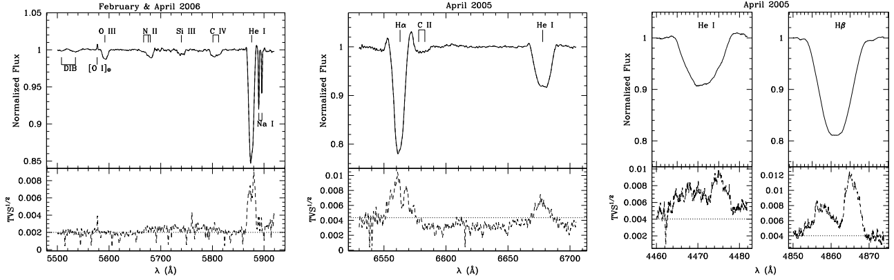
Fig. 1. Average spectrum ( top ) and temporal variance spectrum (TVS, bottom ) computed from the green, red and SPM spectra taken in February + April 2006 ( left panel ), April 2005 ( middle ) and April 2005 ( right ) respectively. The dotted lines yield the 99% significance level for the variability evaluated following the approach of Fullerton et al. (1996).
