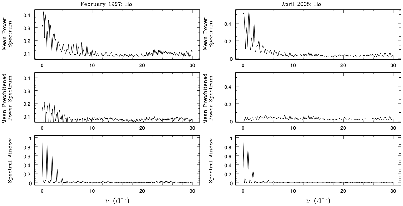
Fig. 7. Same as Fig. 4 but for the H \alpha line: February 1997 ( left ) and OHP April 2005 ( right ). The power spectra are averaged over the wavelength domain from 6540 to 6580 Å. The frequencies used for prewhitening are 0.30, 6.94 and 6.26 d ^{-1} for the February 1997 data and 1.18, 3.09 and 1.67 d ^{-1} for the April 2005 campaign.
