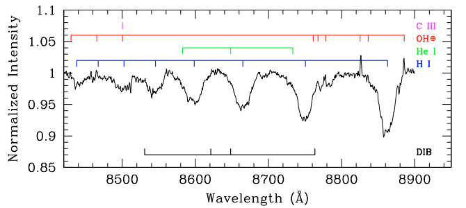
Fig. 2. Mean spectrum of HD 93521 over the 8420–8900 Å wavelength domain. The ions responsible for the lines (either stellar, or telluric in the case of the OH emissions) are indicated above the spectrum, whilst the diffuse interstellar bands (DIBs) are indicated below.
