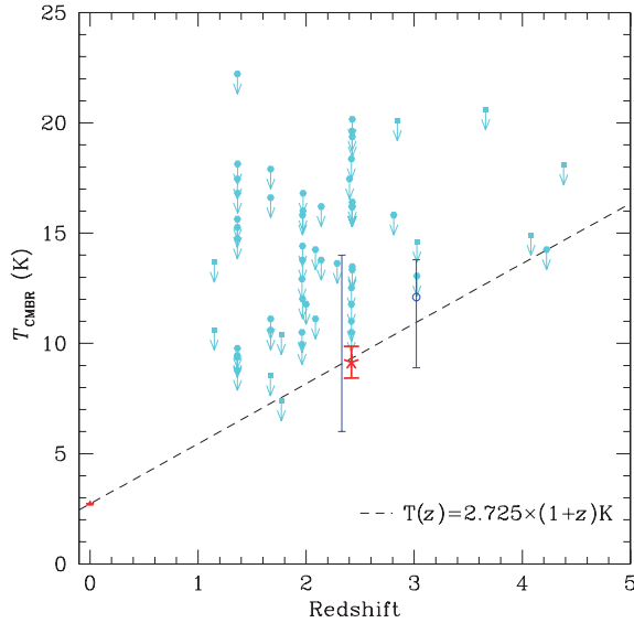
Fig. 5. Measurements of T(\text{CMBR}) at various z . The star with error bars is for the measurement based on CO presented here. Our earlier measurement using fine-structure lines of neutral carbon, 6.0 < T_{\text{CMBR}} < 14.0 K, at z = 2.33771 is indicated by the long vertical bar (Srianand et al. 2000). Measurement by Molaro et al. (2002) is marked by an open circle. Upper limits are measurements using C I or C II* from the literature (squares) and using C I from our UVES sample (hexagons). The dashed line is the prediction from the hot big-bang theory, T_{\text{CMBR}}(z) = T_{\text{CMBR}}(z=0) \times (1+z) . T_{\text{CMBR}} measurement at z=0 is based on the COBE determination (Mather et al. 1999).
