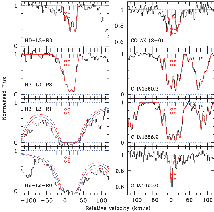
Fig. 1. A sample of molecular and heavy element absorption lines associated with the damped Lyman- \alpha system toward SDSS J143912.04+111740.5. The normalized flux is given on a velocity scale with the origin at z_{\text{abs}} = 2.41837 . Smooth curves in each panel show our Voigt profile fits to the data. The dashed profiles shown for J \leq 1 H 2 lines are the 1\sigma ranges. Tick marks in each panel indicate the locations of the 6 components that are used to fit the J = 3 H 2 absorption lines. The symbol “CO” marks the locations of two components detected in S I and CO.
