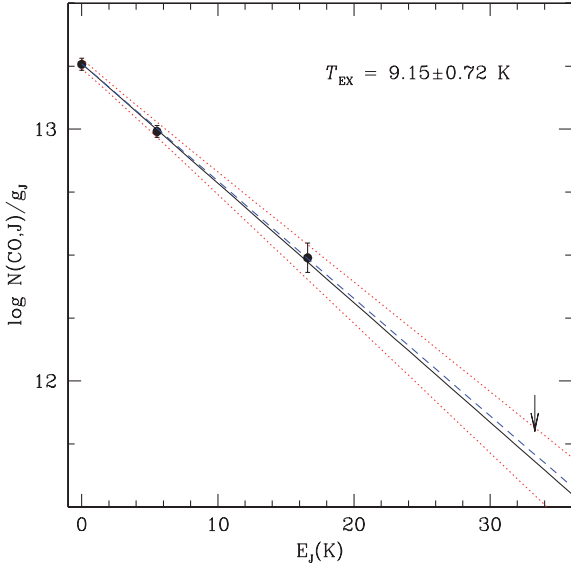
Fig. 3. The CO excitation diagram. A straight line with slope 1/(T_{\text{ex}} \ln 10) indicates thermalization of the levels. The diagram is given for the main CO component at z_{\text{abs}} = 2.41837 . The three lines give the mean and 1\sigma range obtained from T_{01} , T_{02} , and T_{12} . The diagram is compatible with thermalization by a black-body radiation of temperature 9.15 \pm 0.72 K when T_{\text{CMBR}} = 9.315 \pm 0.007 K (long dashed line) is expected at z_{\text{abs}} = 2.4185 from the hot big-bang theory.
