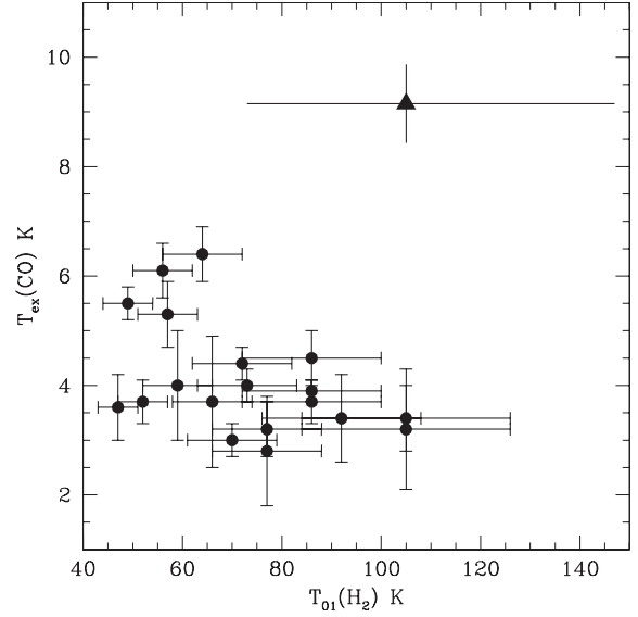
Fig. 4. Comparison of rotational excitation temperatures of CO and \text{H}_2 . Filled circles are for the measurements from Galactic diffuse ISM (Burgh et al. 2007). The filled triangle is for our measurement at z = 2.4183 towards SDSS J143912.04+111740.5.
