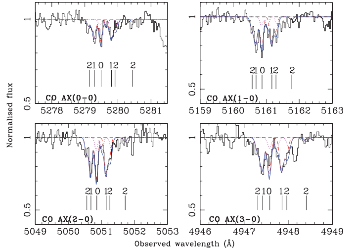
Fig. 2. Voigt profile fits to 12 CO A-X bands detected at z_{\text{abs}} = 2.4185 towards SDSS J143912.04+111740.5. The vertical lines mark the locations of CO absorptions from different J levels at the redshift of the main component. The profiles in dashed and dotted lines are, respectively, for the first and second components (at z_{\text{abs}} = 2.41837 and 2.41847 ) and the total profile is shown in solid line.
