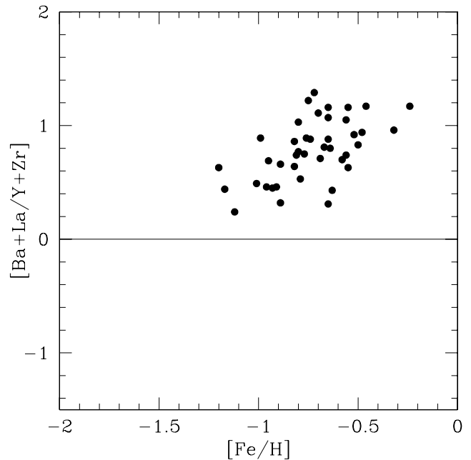
Fig. 13. Observed abundance ratios [hs/l_s] = [\text{Ba}+\text{La}/\text{Y}+\text{Zr}] .
