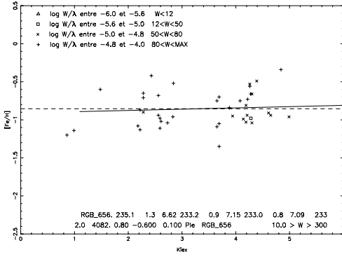
Fig. 2. Example of the temperature calculation for RGB_656: [Fe I/H] vs. \chi_{\text{exc}} .
