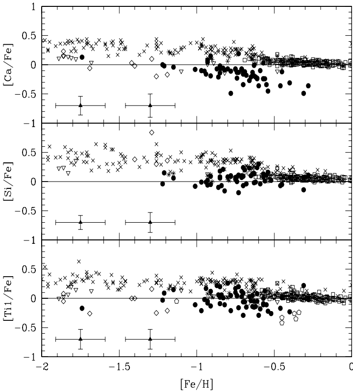
Fig. 8. Abundance distributions for the inner disk LMC stars: [\alpha/Fe] vs. [Fe/H] (dots). LMC samples are depicted with polygons (downward-pointing triangles – Hill et al. 2000; pentagons – Smith et al. 2002; diamonds – Johnson et al. 2006); and the remaining symbols are data for the Galactic stars (crosses – Fulbright 2000; open squares – Reddy et al. 2003; asterisks – Nissen & Schuster 1997). Error bars depict a) leftmost side of the plots – errors due to stellar parameter uncertainties (Table 3), and b) more to the right side – errors associated with the abundance analysis – for those derived from the EW , is the mean error of Tables 5–7; for those elements with abundances derived from spectrum synthesis, the value is described in Sect. 4.
