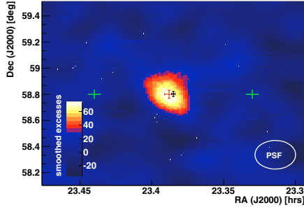
Fig. 2. Sky map around the position of Cas A. A lower cut in SIZE of 400 PE was applied. The green crosses mark the 2 wobble positions. The red cross indicates the MAGIC best fit position. The black cross marks the HEGRA source position, which is within 1 standard deviation from the MAGIC one. The bars of the crosses for both the MAGIC and HEGRA marks correspond to 1 sigma statistical errors.
