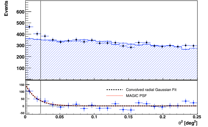
Fig. 1. The upper panel shows the distributions of \theta^2 (measured in degree 2 ) in the direction of the source (black dots) and anti-sources (blue shaded histogram). A lower SIZE cut of 400 PE was applied. The lower panel shows the \theta^2 distribution after background subtraction. The vertical line shows the optimum angular cut. The red function corresponds to the telescope PSF and is derived from Crab nebula data taken in the same observational conditions as those for Cas A. The black distribution is the result of a Gaussian fit to the excess distribution.
