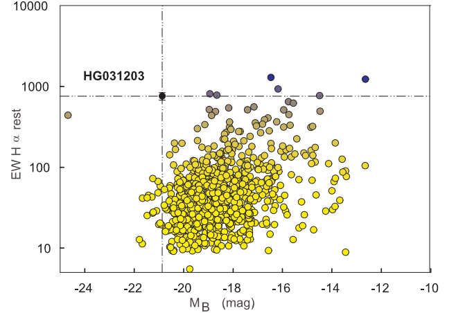
Fig. 9. Equivalent width at rest of the H\alpha line for HG 031203 and for a complete sample of normal star-forming galaxies of the local universe (KPNO International Spectroscopic Survey of galaxies, Salzer et al. 2000) as a function of absolute B -band magnitude. KISS data are not extinction corrected.
