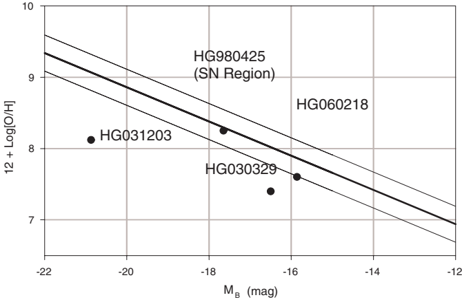
Fig. 8. Metallicity–luminosity relationship for KISS galaxies (thick line) and for local LGRB HGs. For HG 030329 and HG 060218 we applied the metallicity conversion of L. J. Kewley & S. L. Ellison (2007, in preparation) to the R_{23} estimates of Table 9. Thin lines mark the rms 0.25 dex deviation of residuals about the fit. We refer the reader to Melbourne et al. (2004) for details.
