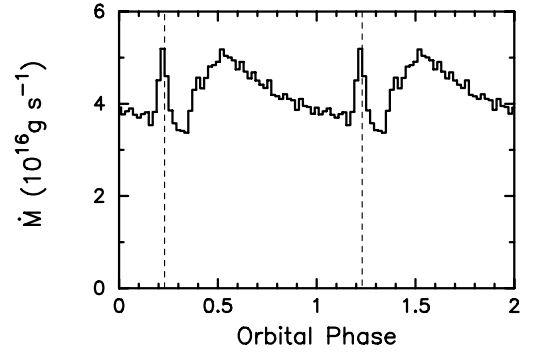
Fig. 2. Phase dependence of the accretion rate onto the compact object. To reduce the fluctuation noise, the data is averaged over three orbital period. The vertical dashed lines denote periastron passage at phase 0.23.
