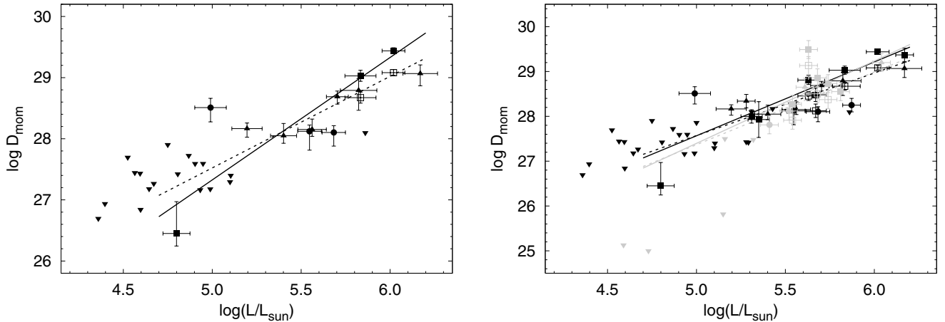
Fig. 3. Modified wind momentum – luminosity distribution for SMC stars. The symbols have the same meaning as in Fig. 1. To construct the uncorrected and clumping corrected empirical WLR (solid and dashed line) the dwarf NGC346 033 at \log L_*/L_\odot \approx 5.0 was not taken into account as the scaling of the escape velocity resulted in an anomalously high wind velocity. In Table 3 the fit coefficients for the individual relations are listed. Left: stars analysed by Mokiem et al. (2006) an automated fitting method. Right: total SMC sample. It turns out that the WLR is strongly influenced by the objects with \log L_*/L_\odot < 5.3 . This is shown by the grey lines, which correspond to the empirical WLRs calculated ignoring these objects. For establishing the empirical \dot{M}(Z) as well as for the comparison with theory we will use the latter set of WLRs. Upper limits were not considered in determining any of the best fits.
