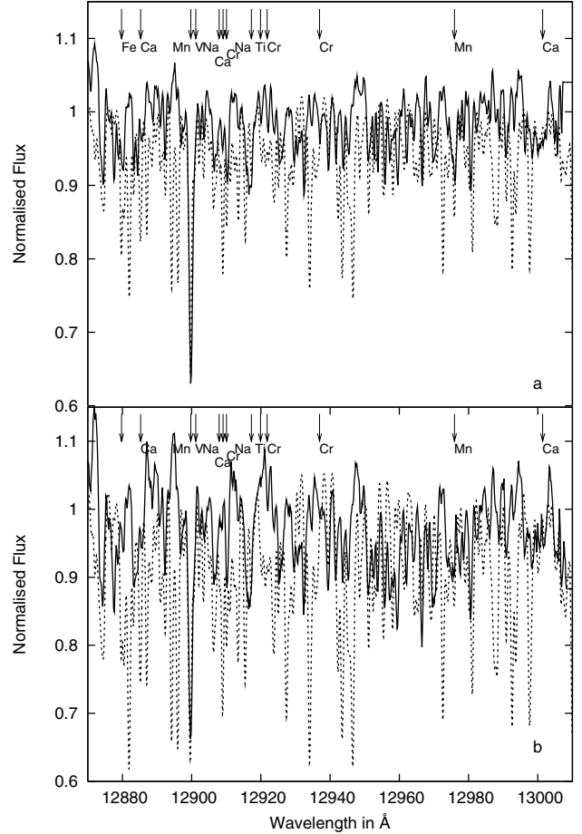
Fig. 3. a) The observed GJ406 (M6 V) and b) 2M0140+27 (M8.5 V) spectra (solid line) compared to the 2800/5.0/0.0 and 2500/5.0/0.0 synthetic spectra, computed using molecular line lists of \text{H}_2\text{O} (BT2), TiO, FeH, CrH (dotted line).
