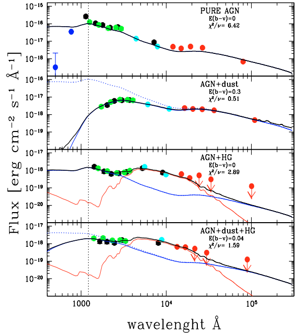
Fig. 4. Four examples of different decompositions of the observed SEDs of our objects. Photometric data below \lambda < 1216 Å in the rest-frame are considered lower-limits. The four fits shown in this figure correspond, from top to bottom, to pure-AGN, dust-extinguished AGN, AGN and host galaxy, dust-extinguished AGN and host galaxy. The dotted line corresponds to the AGN template before the application of the extinction law, while the solid blue line corresponds to the same template taking extinction into account. The red line (third and fourth panel) corresponds to the galaxy template and, finally, the black line is the resulting best fit to the SED. Arrows correspond to 5\sigma upper limits in case of non detection in the IR.
