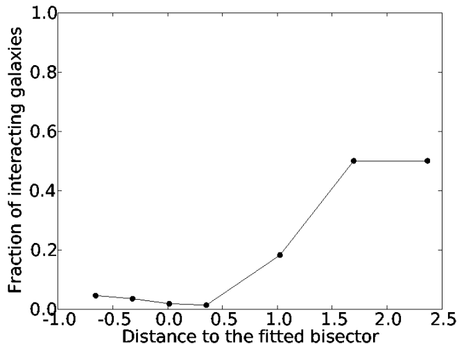
Fig. 12. The fraction of interacting galaxies is shown as a function of the distance to the fitted bisector (calculated only including the similar size neighbours within 0.5 Mpc of each CIG galaxy).
