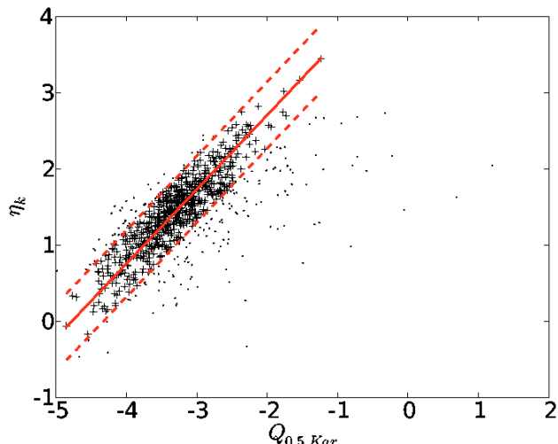
Fig. 11. Local number density vs. tidal strength ( Q_{0.5, \text{Kar}} ). The final bisector fit is shown by the plain red line. The dotted red lines represent the final 2\sigma dispersion: the CIG galaxies within these limits are depicted by pluses, the CIG rejected during the successive iterations are shown by points.
