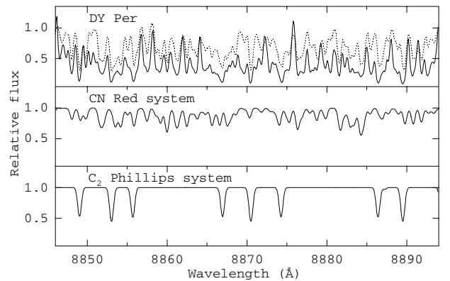
Fig. 12. High-resolution spectrum of DY Per (upper panel) in the spectral region from 8850 to 8890 Å. The dotted line represents the spectrum of cool carbon star U Hya. The synthetic spectra of the CN Red system and the \text{C}_2 Phillips system calculated for typical warm (3700 K) carbon star are given for comparison purposes.
