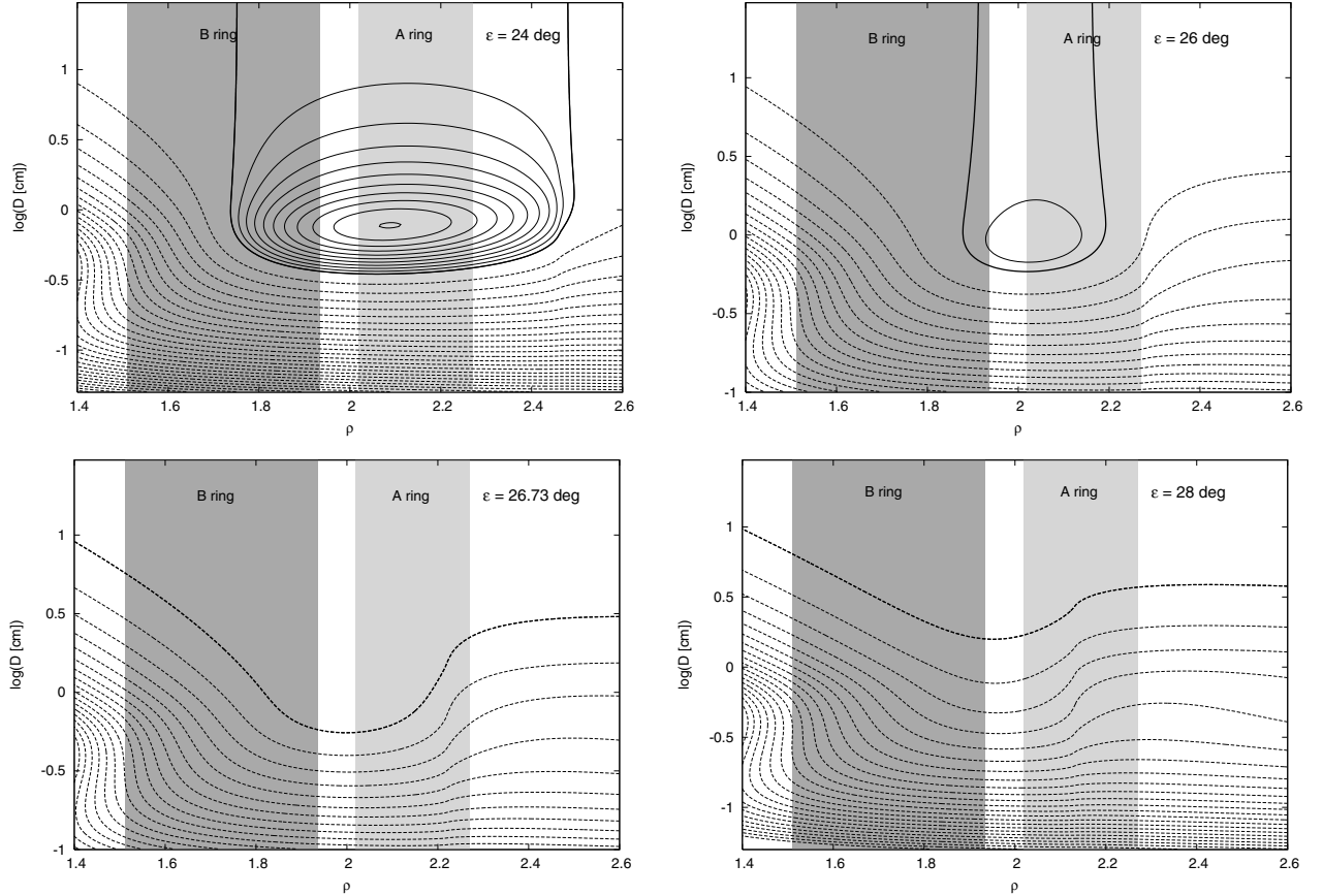
Fig. 4. Isolines of positive (solid) and negative (dashed) values of the mean transverse acceleration [f_{\tau}]_{123} resulting from composition of thermal and P-R effects in the plane of distance from Saturn ( \rho in planetary radii) and size of the ring particle ( D in cm). The four plots correspond to four possible values of Saturn's obliquity: (i) \varepsilon = 24^\circ (left and top), (ii) \varepsilon = 26^\circ (right and top), (iii) \varepsilon = 26.73^\circ (left and bottom; current value), and (iv) \varepsilon = 28^\circ (right and bottom). The level curve distance is 0.25 \text{ pm/s}^2 for positive values, and -1 \text{ pm/s}^2 for negative values. In the two top figures the thick solid isoline is where [f_{\tau}]_{123} = 0 \text{ pm/s}^2 , while in the bottom two figures (where no positive [f_{\tau}]_{123} occur) the thick dashed line is for [f_{\tau}]_{123} = -1 \text{ pm/s}^2 . The ring particles are assumed to have the following thermal parameters: bulk density \rho_b = 0.5 \text{ g/cm}^3 , specific heat capacity C = 820 \text{ J/kg/K} , thermal conductivity K = 10^{-4} \text{ W/m/K} and ratio of thermal and optical absorptivity \alpha_1/\alpha_V = 1.33 and \alpha_V = 0.5 . Shaded zones indicate position of the main B and A rings.
