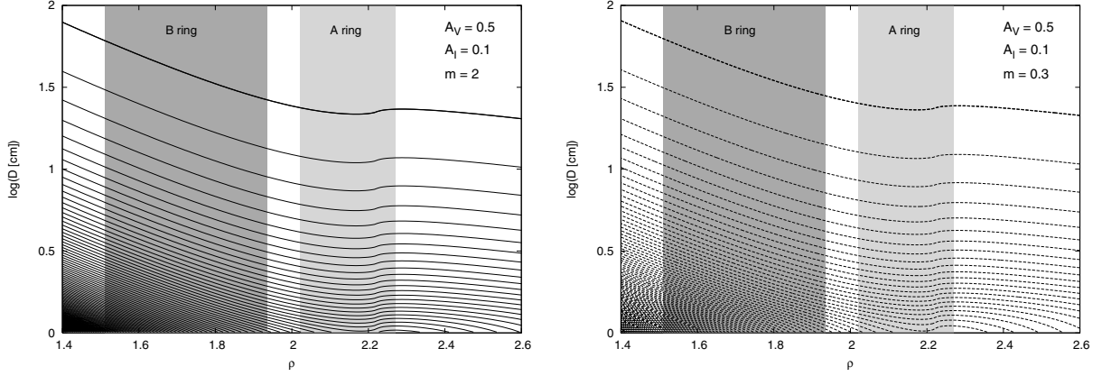
Fig. D.1. The same as in Fig. 6 but now the results assume a population of particles with zero obliquity (such that their spin axes are aligned with the normal to the disk plane). Two values of particle rotation rate are investigated: (i) m = 2 (left), and (ii) m = 0.3 (right). Thermal and optical parameters of icy particles of appropriate to the A ring assumed and the nominal value \varepsilon = 26.73^\circ of Saturn’s obliquity. Particles with m > 1 at any planetocentric distance migrate outward since the diurnal variant of the planetary Yarkovsky effect is stronger than the corresponding component of the Yarkovsky-Schach effect. However, the situation reverses for the extreme case m < 1 . We plot isolines of [f_\tau]_{12} with a constant step 1 \text{ pm/s}^2 (starting with the bold curve corresponding to [f_\tau]_{12} = 1 \text{ pm/s}^2 in the left panel and [f_\tau]_{12} = -1 \text{ pm/s}^2 in the right panel). Solid/dashed curves apply to positive/negative [f_\tau]_{12} values.
