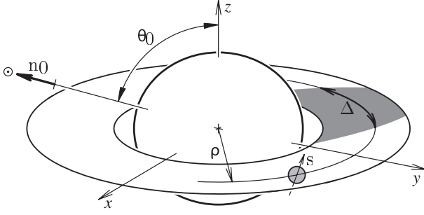
Fig. 1. Ring geometry, parameters of the particle orbit about Saturn and other quantities introduced in the text: \mathbf{n}_0 is the unitary vector toward the Sun, tilt from the Saturn spin axis by \theta_0 , \mathbf{s} is the unitary spin axis of the particle and \rho radius of its planetocentric orbit. The shaded zone on the ring plane indicates shadow cast by the planet. For given \rho and \theta_0 , the angular width \Delta of the shadow along the orbit is given by Eq. (10).
