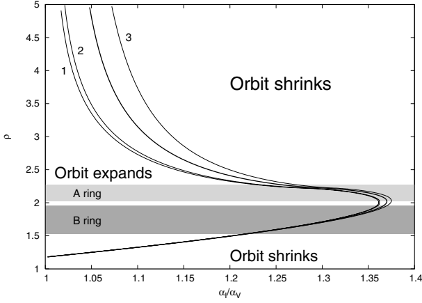
Fig. E.1. Distance from Saturn where the total thermal torque on the orbital motion of ring particles is zero as a function of ratio between its absorptivity in thermal \alpha_1 and optical \alpha_v bands. Seasonal components of the Yarkovsky and Yarkovsky-Schach effects were taken into account. For sake of illustration we assume particle of diameter D = 1 cm, bulk density \rho_b = 0.5 g/cm 3 and specific thermal capacity C = 820 J/kg/K. The light curves correspond to three values of thermal conductivity: (i) K = 10^{-4} W/m/K (label 1), (ii) K = 10^{-2} W/m/K (label 2), and (iii) K = 1 W/m/K (label 3). The bold curve was calculated from approximate conditions (E.2) and (E.3). Position of the A and B rings is shown by the shaded zones. For large enough \alpha_1/\alpha_v ratio the approximate method provides a very good means to compute the no-torque orbits independently on the ring particle thermal parameters and size. When \alpha_1/\alpha_v \leq 1 (physically unlikely case) all ring orbits would gain orbital momentum.
