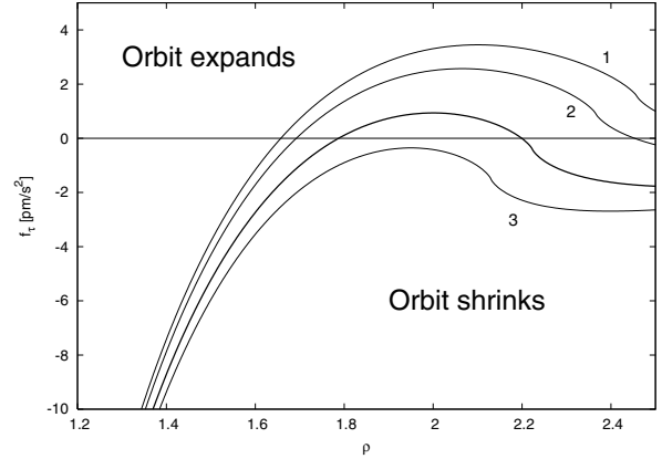
Fig. 2. Long-term mean thermal transverse acceleration (in pm/s 2 ) for D = 1 cm ring particles as a function of the planetocentric distance \rho (in planet's radii). We assume bulk density \rho_b = 0.5 g/cm 3 , specific thermal capacity C = 820 J/kg/K and thermal conductivity K = 10^{-4} W/m/K. Optical and thermal absorptivities are \alpha_V = 0.5 and \alpha_I = 0.665 . Four different curves are for different assumptions about Saturn's obliquity \varepsilon : (i) 24° (label 1), (ii) 25° (label 2), (iii) 26.73° (the current value; thick line), and (iv) 28° (label 3).
