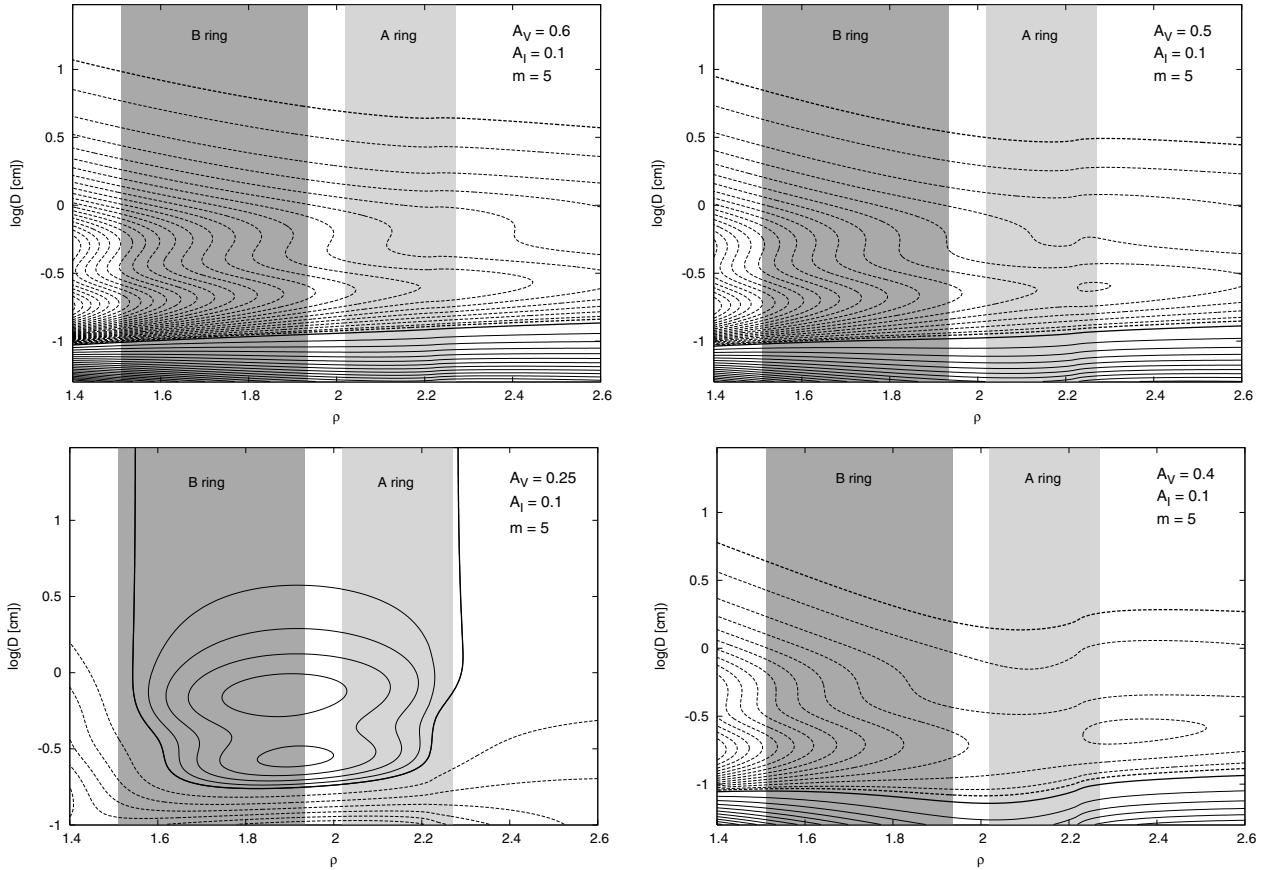
Fig. 6. The same as in Fig. 5 but now the results include effects of the diurnal variants of the thermal forces. All particles are assumed to have a rotation period five times shorter than the revolution period (i.e. m = 5 ). The four panels are again appropriate for Saturn's B ring ( top left ), A ring ( top right ), C ring ( bottom left ) and Cassini division ( bottom right ). Nominal value \varepsilon = 26.73^\circ of Saturn's obliquity and low conductivity K = 10^{-4} W/m/K are assumed here. Dashed are isolines of negative [f_r]_{123} values with constant step -3 \text{pm/s}^2 (the bold dashed curves correspond to [f_r]_{123} = -3 \text{pm/s}^2 ). Solid are isolines of positive [f_r]_{123} values with constant step +10 \text{pm/s}^2 (the bold solid curve on the left and bottom panel is [f_r]_{123} = 0 \text{pm/s}^2 ) with the exception of the bottom left panel where the step is +1 \text{pm/s}^2 only.
