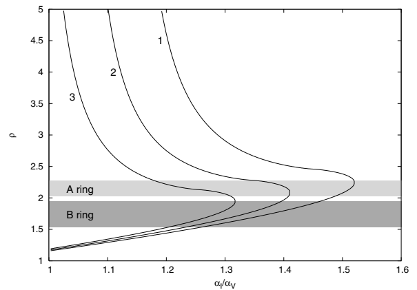
Fig. 3. Distance from Saturn where zero mean thermal torque [f_{\tau}]_{123} = 0 applies on the orbital motion of ring particles as a function of ratio between their absorptivity in thermal \alpha_I and optical \alpha_V bands. We assume particles of diameter D = 1 cm, bulk density \rho_b = 0.5 g/cm 3 , specific thermal capacity C = 820 J/kg/K and thermal conductivity K = 10^{-4} W/m/K. Current position of the A and B rings is shown by the shaded zones. The three curves are for three possible values of Saturn's obliquity \varepsilon : (i) 24° (label 1), (ii) 26° (label 2), and (iii) 28° (label 3).
