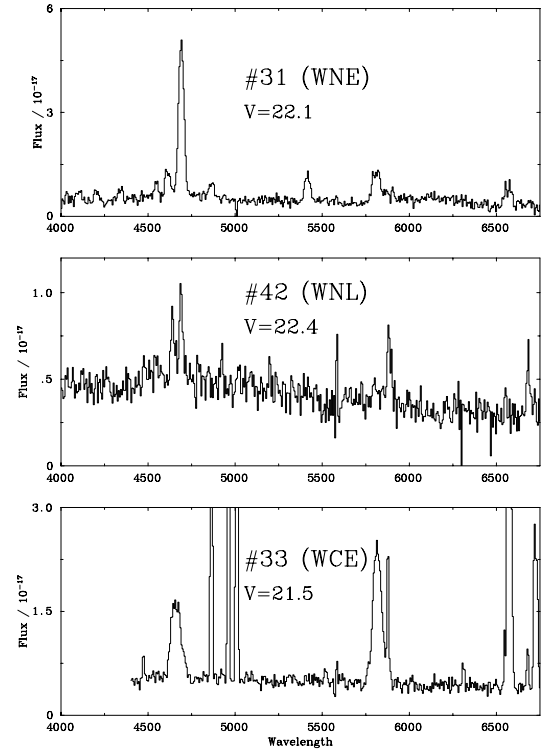
Fig. 1. VLT/FORS2 spectroscopy of three new WR stars. Narrow emission lines in the spectrum of #33 are from an associated H II region.
