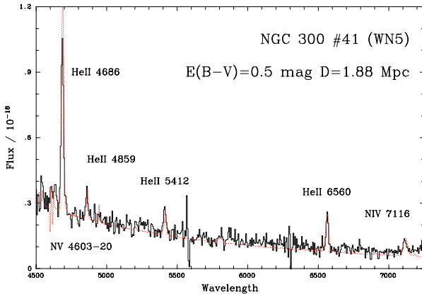
Fig. 5. Spectroscopic comparison between the de-reddened VLT/FORS2 spectrum of NGC 300 #41 and the theoretical non-LTE model (dotted-lines) discussed in the text.
