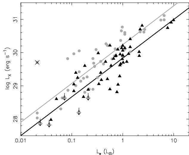
Fig. 1. The dependence of X-ray luminosity upon stellar luminosity for the accreting (black triangles) and non-accreting (grey circles) T Tauri stars in Taurus-Auriga observed by XMM-Newton . The black and grey lines show the best-fitting correlations for accretors and non-accretors, respectively, found using the EM algorithm in ASURV (Telleschi et al. 2007). Open symbols and downward-pointing arrows mark upper limits. The cross shows KPNO-Tau 8, which was excluded from the fitting.
