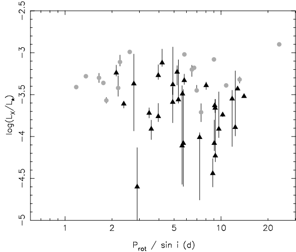
Fig. 5. The ratio of X-ray and stellar luminosities plotted as a function of rotation period for T Tauri stars in Taurus-Auriga observed by XMM-Newton with measured v \sin i . Rotation periods have been calculated from v \sin i and the stellar radius and the plotted values include an unknown factor \sin i and are therefore upper limits. Triangles denote accretors and circles mark non-accretors.
