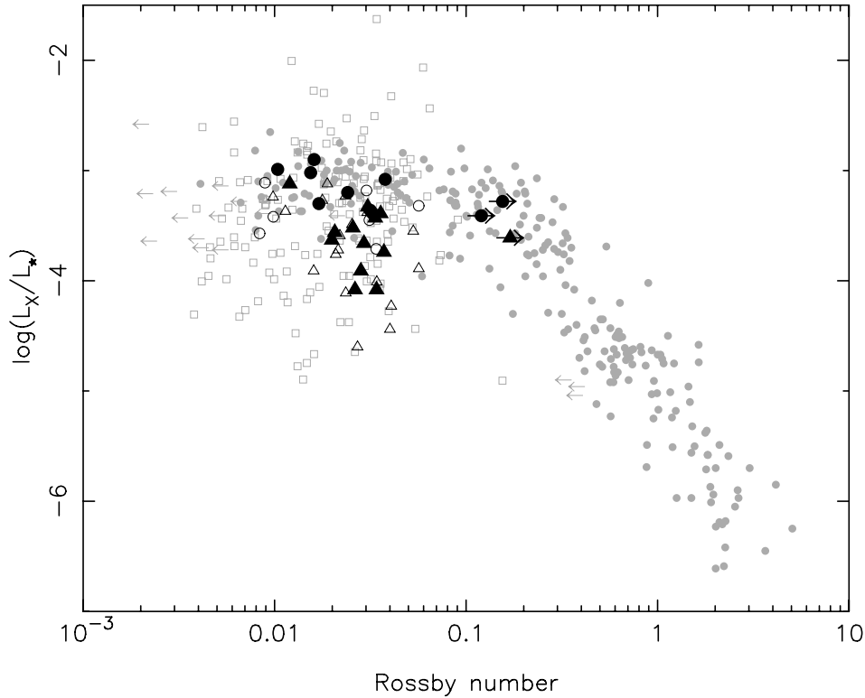
Fig. 7. The ratio of X-ray and stellar luminosities plotted as a function of Rossby number. Grey filled circles show late-type main sequence stars studied by Pizzolato et al. (2003); grey open squares show T Tauri stars in the Orion Nebula Cluster studied by Preibisch et al. (2005); black circles and triangles show, respectively, non-accreting and accreting T Tauri stars in Taurus-Auriga in the present study. The filled black symbols show stars with measured photometric rotation periods; the open black symbols have periods derived from v \sin i measurements and are effectively upper limits to the Rossby number. The grey leftward-pointing arrows represent periods derived from v \sin i measurements in Pizzolato et al. (2003). The black rightward-pointing arrows show cases where only upper limits to the convective turnover time could be estimated.
