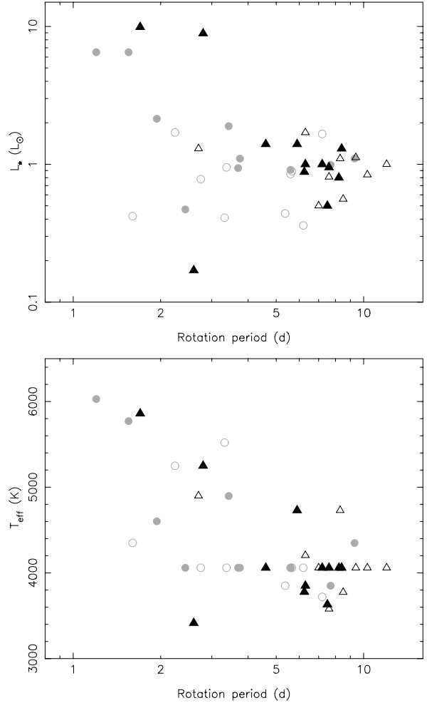
Fig. 4. The stellar luminosities ( top ) and effective temperatures ( bottom ) of T Tauri stars in Taurus-Auriga with measured photometric rotation periods. Black triangles indicate accretors and grey circles mark non-accretors. Filled symbols denote stars observed by XMM-Newton in the present survey; unfilled symbols denote additional stars observed by ROSAT (Stelzer & Neuhäuser 2001).
