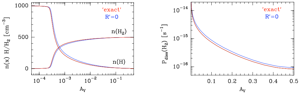
Fig. 3. Impact of the new “exact” radiative transfer computation compared to an alternative approach that assumes R' = 0 (Le Petit et al. 2006). Grain properties are uniform in all the cloud (MRN). Left panel: \text{H}/\text{H}_2 transition. Right panel: \text{H}_2 photodissociation rate as a function of cloud depth. A cloud with a density of n_H = 10^3 \text{ cm}^{-3} , a total extinction depth of A_V = 1 and illuminated at both sides by the mean ISRF is considered. These results show that for the case of uniform dust grain properties the error associated with R' = 0 assumption is small.
