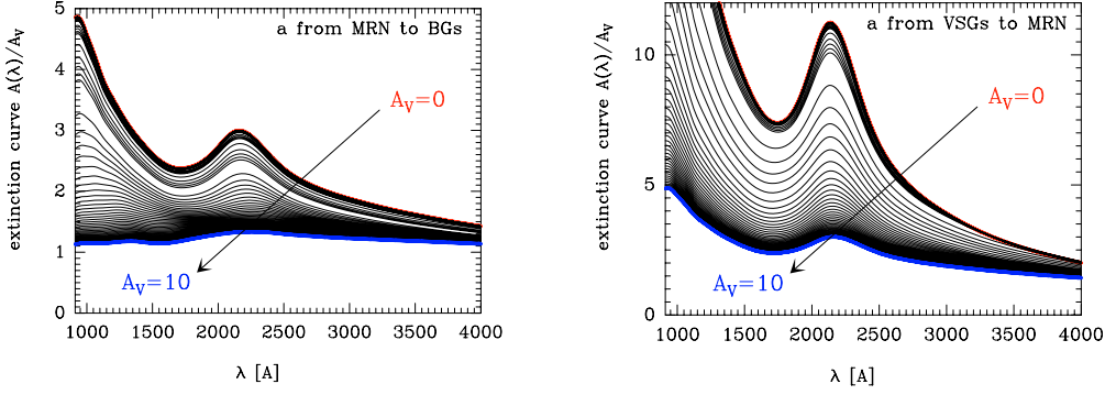
Fig. 5. Resulting extinction curves as a function of wavelength (only the FUV range is shown) and cloud depth (the red curve corresponds to the cloud edge A_V = 0 and the blue curve to A_V = 10 ) for the “MRN to BGs” (left) and “VSGs to MRN” (right) examples respectively.
