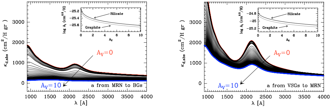
Fig. 6. Dust mass absorption coefficients (per gas gr) as a function of wavelength and cloud depth (the red curve corresponds to the cloud edge A_V = 0 and the blue curve to A_V = 10 ) for the “MRN to BGs” (left) and “VSGs to MRN” (right) examples respectively. The different grain material A_i coefficients required to keep a constant gas-to-dust mass ratio are also shown as a function of A_V in the small insets.
