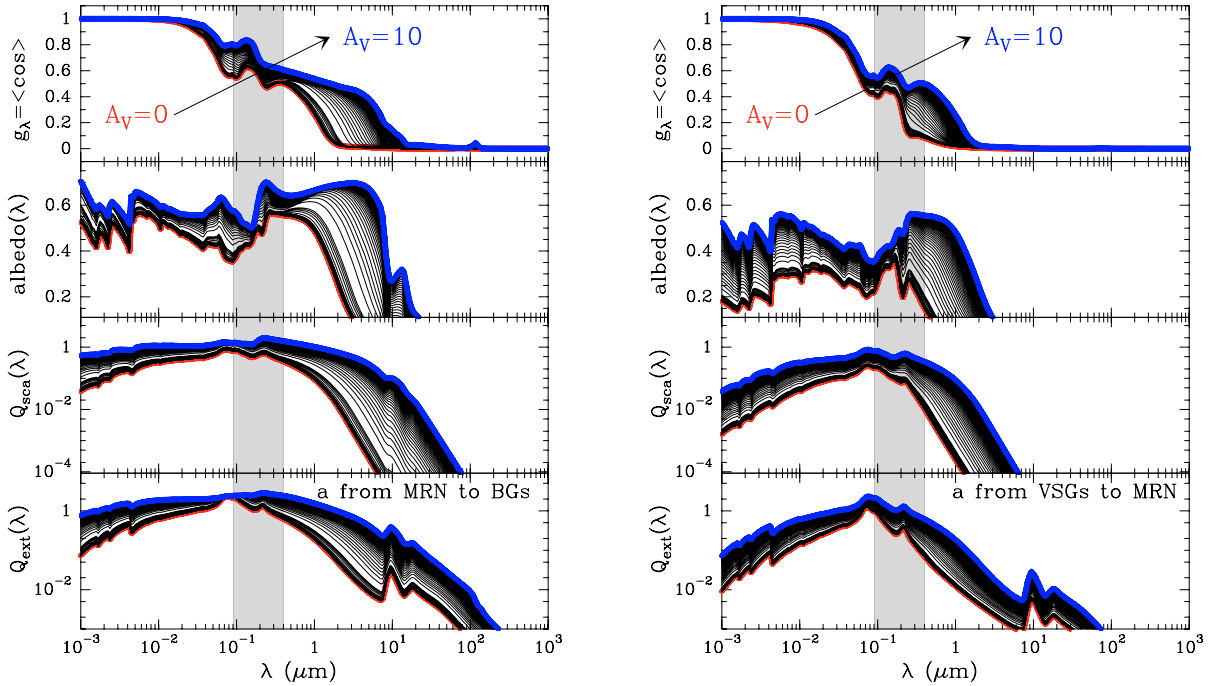
Fig. 4. Grains mixture optical parameters as a function of wavelength and cloud depth (the red curve corresponds to the illuminated cloud edge A_V = 0 and the blue curve to the center of the cloud at A_V = 10 ) for the “MRN to BGs” (left) and “VSGs to MRN” (right) examples respectively. The shaded region shows the spectral region taken into account in the FUV radiative transfer.
