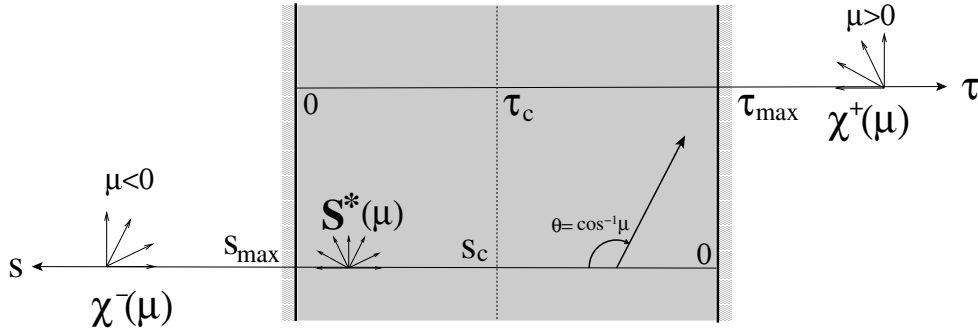
Fig. 1. Adopted geometry and sign conventions for a cloud with embedded sources of photons S^*(\mu) and illuminated at both surfaces by \chi^\pm(\mu) .
