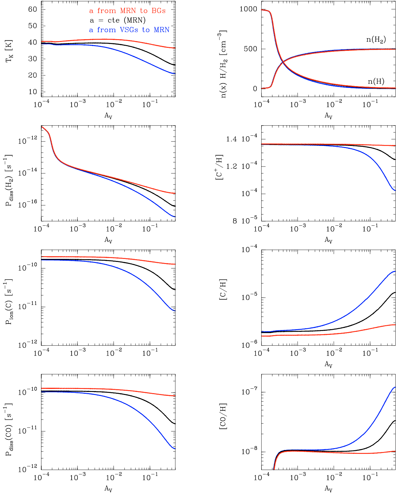
Fig. 10. Same as Fig. 9 for a cloud with n_H = 10^3 \text{ cm}^{-3} , a total extinction depth of A_V = 1 and illuminated at both sides by the the mean ISRF. Dust grains grow according to Eq. (54) with A_V^c = 1.086 \tau_V^c = 0.5 .
