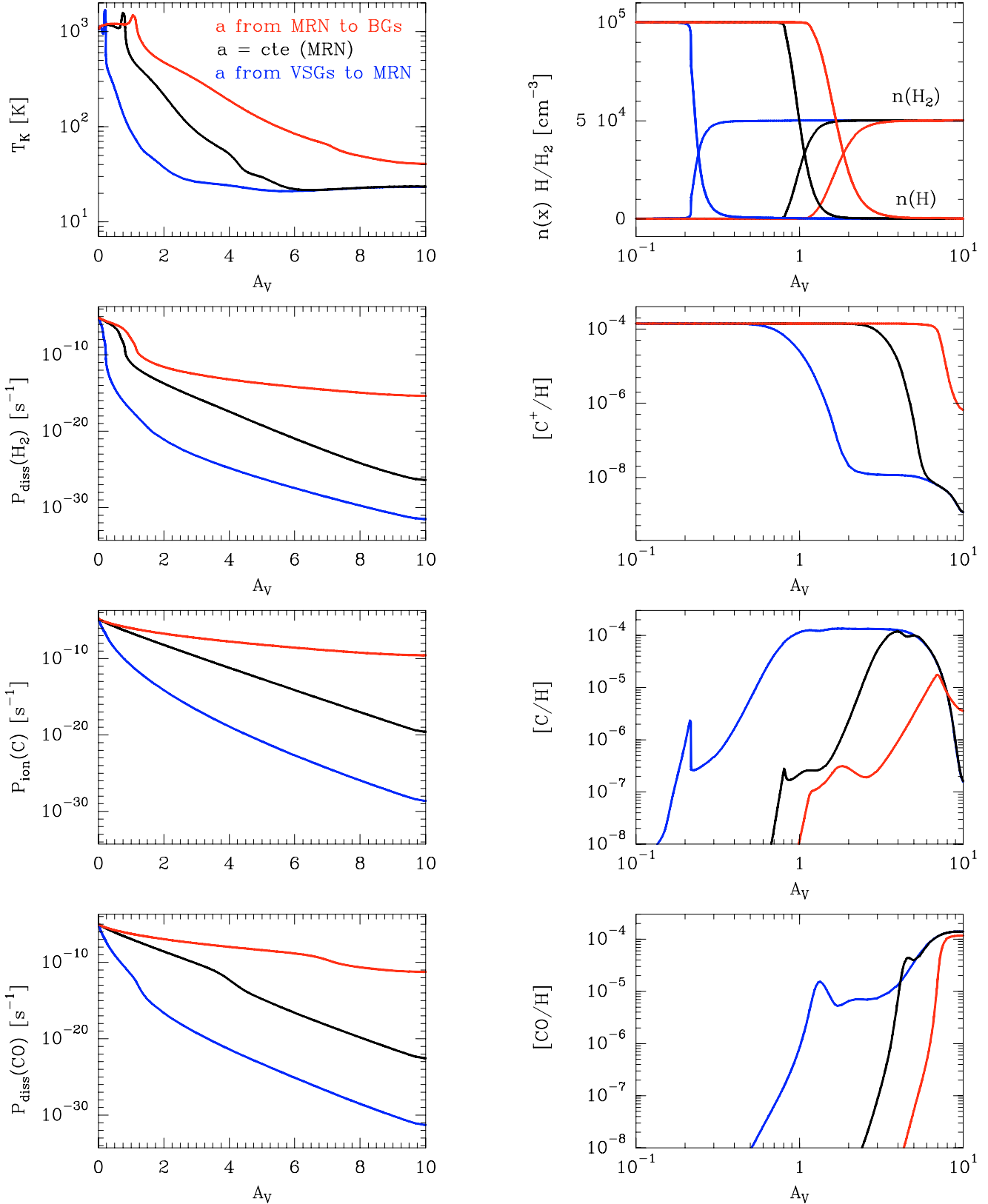
Fig. 9. Impact of the different FUV radiative transfer models on the kinetic temperature, H_2 photodissociation rate, C photoionization rate and CO photodissociation rate (left column), H/H_2 transition and C^+/C/CO abundances (right column). A cloud with a density of n_H = 10^5 \text{ cm}^{-3} , a total extinction depth of A_V = 20 and illuminated at both sides by 10^5 times the mean ISRF is considered. Although not clearly seen in these boxes, all physical parameters show an horizontal tangent at A_V = 10 , consistent with their null variation with respect to the depth position at half cloud (as expected for a symmetrically illuminated cloud).
