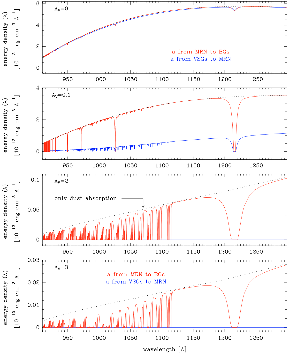
Fig. 8. Radiative transfer models for a cloud with a total extinction of A_V = 20 and a density of n_H = 10^5 \text{ cm}^{-3} , illuminated at both sides by 10^5 times the mean ISRF. Part of the resulting FUV spectra ( \sim 912\text{--}1300 \text{ \AA} ) at different extinction depths: A_V = 0 (cloud surface), A_V = 0.1 , A_V = 2 and A_V = 3 are shown in each box. In each panel, the red (blue) curve corresponds to the “MRN to BGs” (“VSGs to MRN”) example.
