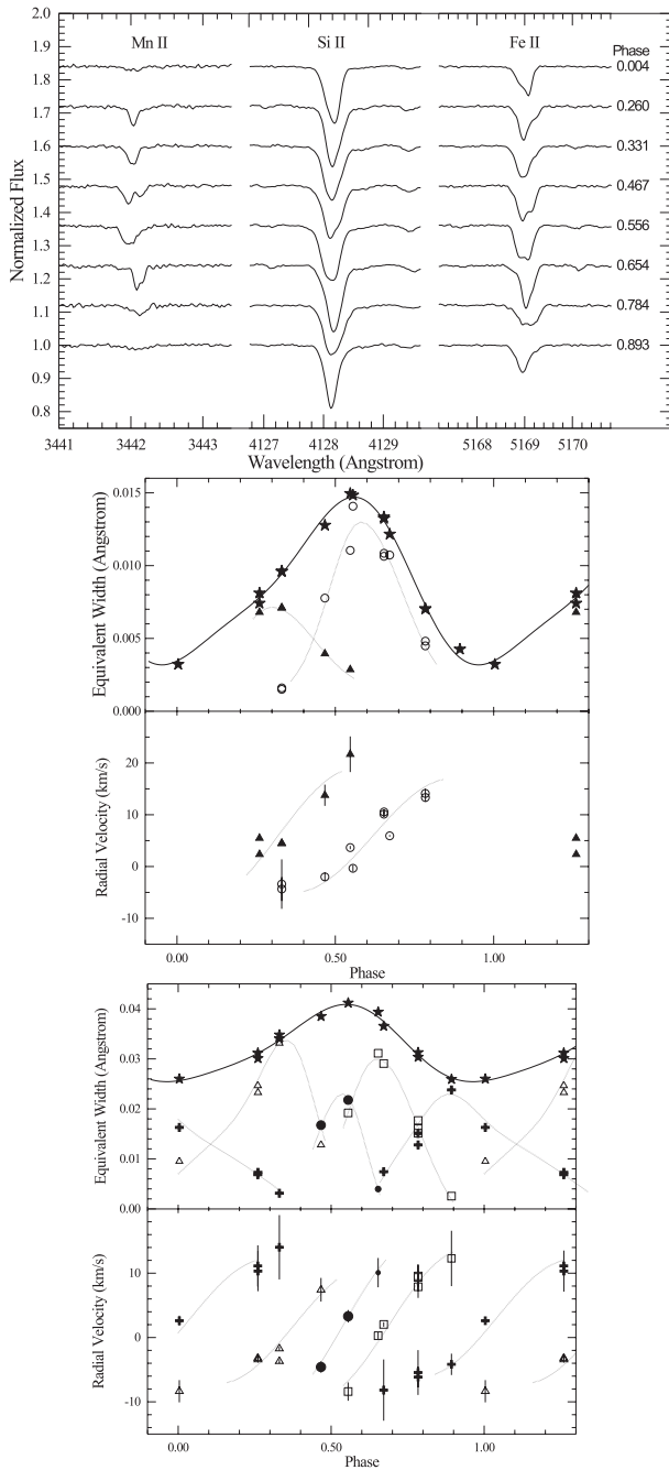
Fig. 3. Upper panel: variations of line profiles of Mn II \lambda 3442 , Si II \lambda 4128 and Fe II \lambda 5169 over the rotation period. Middle panel: phase dependencies of the equivalent width measured by direct integration of the whole profile of the Mn II line at \lambda 3442 (filled stars), and of the equivalent widths measured for split line components (filled triangles and open circles) by fitting multiple Gaussians. The radial velocities corresponding to two Mn II spots are presented in the lower half. Lower panel: the equivalent widths and radial velocities for Fe II \lambda 5169 measured in the same way as for Mn II \lambda 3442 . The surface distribution of Fe II can be represented by four spots crossing the center of the visual disk at the phases 0.35, 0.55, 0.7 and 0.95.
