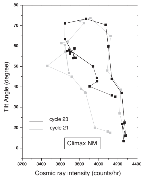
Fig. 15. Comparison of TA vs. GCR intensity (Climax NM) hysteresis curves for solar cycle 21 and 23 (upto September 2006).
