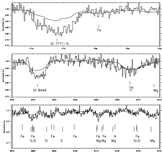
Fig. 1. UVES 2006 spectrum of the oxygen triplet \lambda 7771-5 (top), the O I \lambda 8446 line (middle), containing many lines of the \alpha -elements. We have indicated the major constituents of the line blends, plotting the \alpha -element indicators and identifications below those of the other elements. The overabundance of oxygen is obvious, while the abundances of the other \alpha -elements are comparable with the abundances in HD 156098 (solid line). These three regions correspond almost exactly to the plots of the 1998 Keck-HIRES spectrum (Israelian et al. 1999, Fig. 1), with a few modifications due to UVES inter-order gaps.
