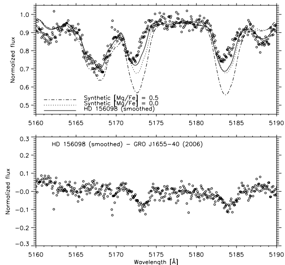
Fig. 2. One of the single UVES 2006 spectrum of GRO J1655-40 (symbols) with the F6IV broadened stellar template of HD 156098 (solid line). Also plotted are two model spectra with [\text{Mg}/\text{Fe}] = 0.0 (dotted line) and [\text{Mg}/\text{Fe}] = 0.5 (dot-dashed line). The apparent wavelength shift is caused by the blending of several lines with the magnesium ones. It has however no influence on Mg abundances. Below are plotted the residuals after subtracting the HD 156098 template spectrum from the GRO J1655-40 spectrum.
