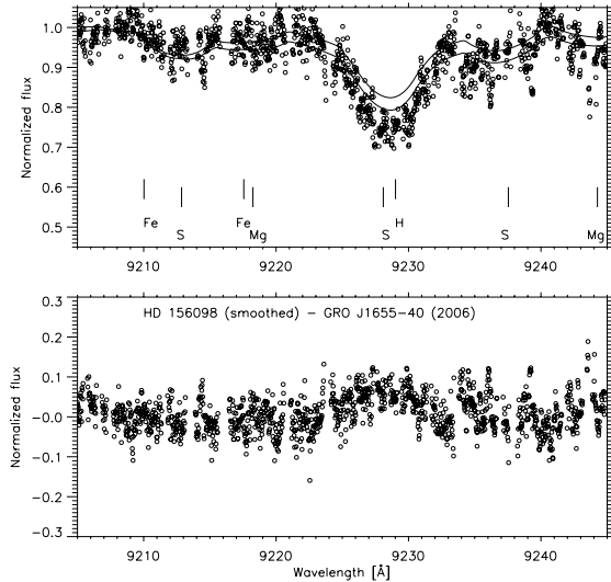
Fig. 3. UVES 2006 spectrum of GRO J1655-40 (symbols) with the F6IV broadened stellar template of HD 156098 (lower continuous line) in the region of the SI triplet. The upper continuous line show the same stellar template, but on which the difference between two acceptable normalizations of the GRO J1655-40 spectrum has been applied. It shows the amplitude of uncertainties in the continuum level in this region, and that in both cases HD 156098 is providing a good match. Below are plotted the residuals after subtracting the HD 156098 spectrum from the best-fitting GRO J1655-40 spectrum.
