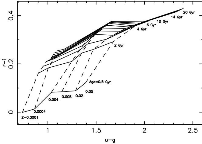
Fig. 3. r-i vs. u-g plane predicted by the low-resolution BC03 model. Lines have the same meanings as in Fig. 1.
