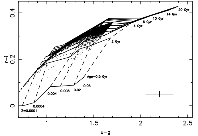
Fig. 5. r-i and u-g colors of 12901 early-type galaxies overlaid onto the theoretical calibration. Error bars show the typical uncertainties. Solid and dashed lines have the same meanings as in Fig. 1.
