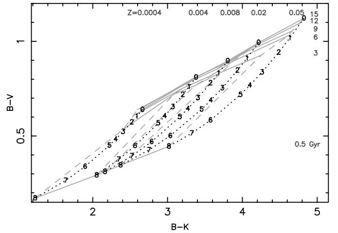
Fig. 6. Changes of B-K and B-V colors when mixing a young stellar population into an old one. The two stellar populations have the same metallicity. Solid and dashed lines are the same as in Fig. 1. Dotted lines represent constant metallicity. Numbers from 0 to 8 show colors of an old population (15 Gyr) mixed with a young population (0.5 Gyr) with different percentages. From 0 to 8, the young population contributes 0, 0.5, 1.0, 2.0, 3.0, 4.0, 10.0, 20.0, and 100 per cent in mass to the total system.
