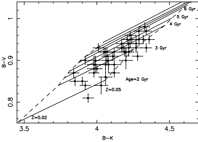
Fig. 4. Colors of 53 elliptical galaxies overlaid onto the B-V vs. B-K plane. Error bars show the uncertainties. Solid and dashed lines have the same meanings as in Fig. 1.
