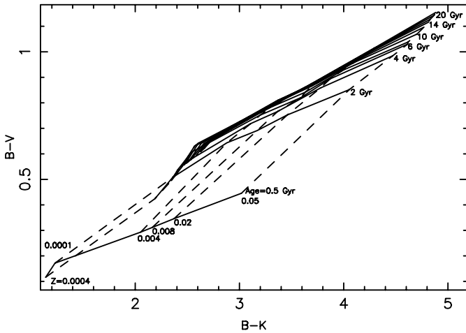
Fig. 1. B - V vs. B - K plane predicted by the high-resolution BC03 model. Solid and dashed lines represent constant age and constant metallicity, respectively.
