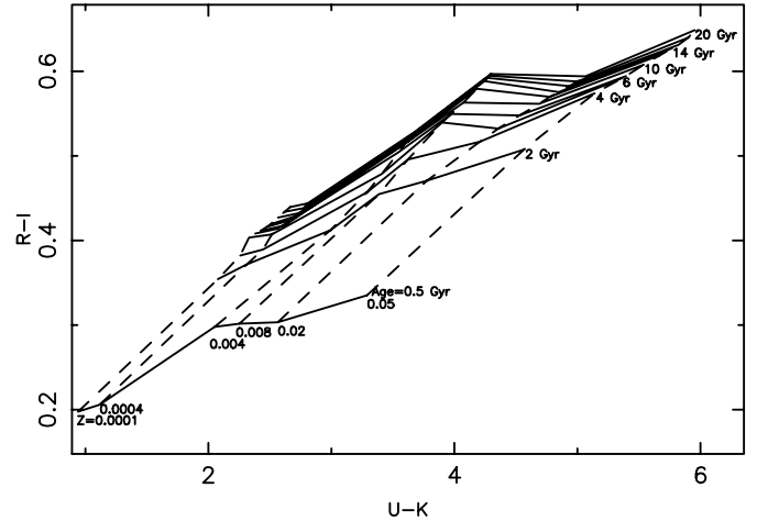
Fig. 2. R - I vs. U - K plane predicted by the low-resolution BC03 model. Lines have the same meanings as in Fig. 1.
