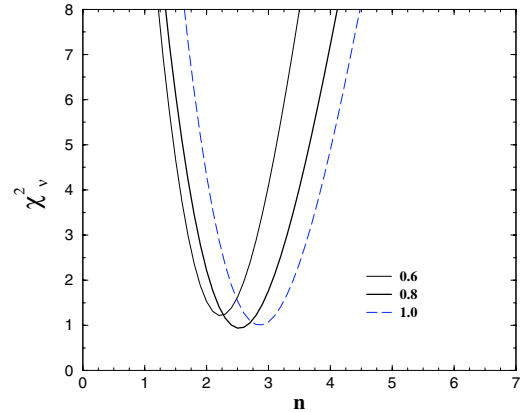
Fig. 7. Reduced \chi^2 versus index n for several hypothesis on the axis ratio (AR = 0.6, 0.8, 1.0).
