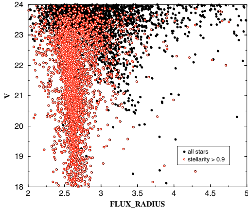
Fig. 1. Visual apparent magnitude versus the extractor parameter FLUX_RADIUS (two different CLASS_STAR selections are shown: filled circles are all objects, open circles are objects with stellarity larger than 0.9).
