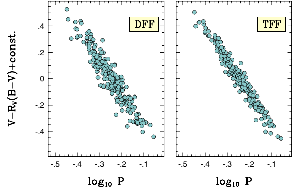
Fig. 10. PLC relations computed from tests on the 248 stars of the basic data set. Test light curves were generated with 30 data points and additive Gaussian noise of 0.03 mag standard deviation. The selective absorption coefficient R_V is set equal to 3.1.
