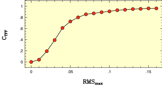
Fig. 6. Completeness function of the TFF method. The symbol C_{\text{TFF}} denotes the relative number of variables that have \text{rms}(\Delta\varphi) < \text{rms}_{\text{max}} . We used the 248 light curves of the basic data set with N = 200 synthetic data points per object and polynomial degree M = 2 .
