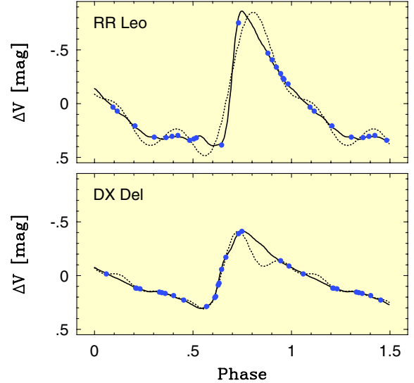
Fig. 7. Examples of the performance of TFF at low data point numbers. Dots, dashed, and continuous lines are for the noiseless synthetic data, DFF, and TFF fits, respectively. The noiseless synthetic data have been obtained by the sparse sampling of the accurate observed light curve.
