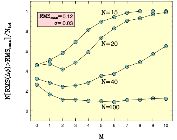
Fig. 4. As in Fig. 3, but with added noise as given in the shaded box.
