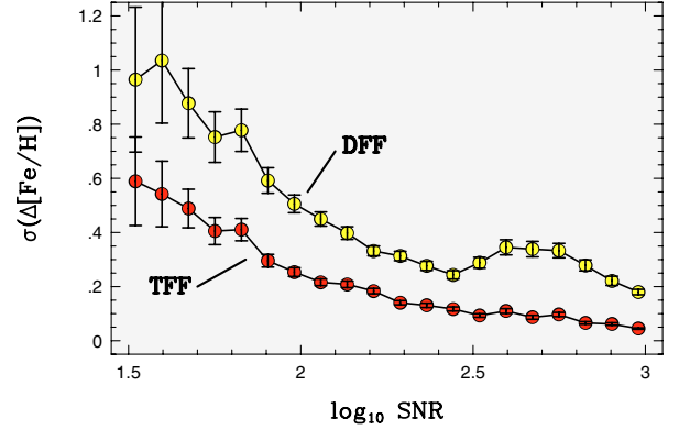
Fig. 8. Standard deviation of the difference between the target and computed Fourier [\text{Fe}/\text{H}] values as a function of SNR . The test was made on the 248 stars of the basic data set. Error bars show the \pm 1\sigma ranges of the means.
