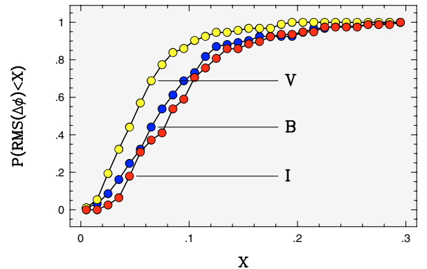
Fig. 9. Empirical probability distribution functions of \text{rms}(\Delta\varphi) for noiseless test signals drawn from samples of RRab stars of different wavebands. All test signals have N = 90 data points. The TFF method with the basic data set (available only in color V ) is used in the computation of \Delta\varphi .
