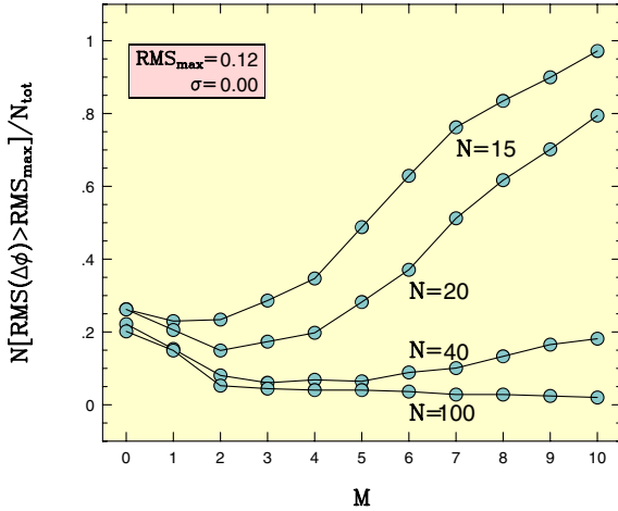
Fig. 3. Dependence of the relative number of poorly fitted targets on the polynomial template degree M and on the number of data points N of the target time series. Tests were made on the basic data set with N_{\text{tot}} = 248 stars. No noise was added to the synthetic data.
