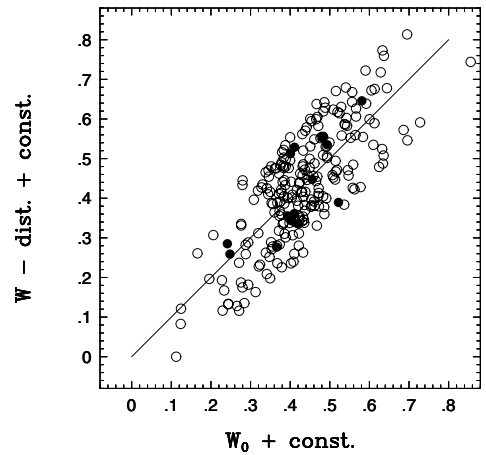
Fig. 13. Correlation between W_0 = -2.33 \log P and W = V - 3.1(B - V) (adjusted to field averages) for 234 RRab stars of selected LMC OGLE fields. The standard deviation of the fit is 0.092 mag, the 1\sigma error of the slope is 0.05. The 45° line is shown for reference. The result have been obtained by TFF with the top 100 most deviating stars clipped. Filled circles denote variables in field #20.
