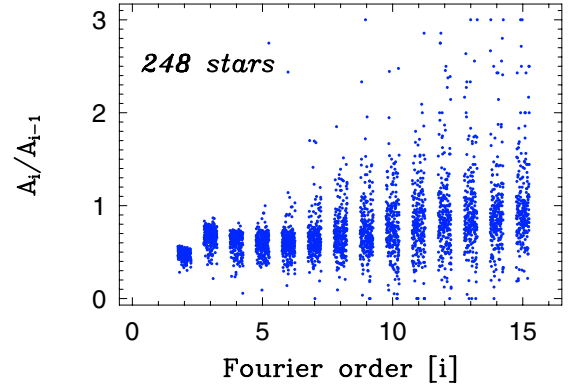
Fig. 1. Amplitude ratios of the successive Fourier components of the 248 RRab stars of the basic data set. For better visibility, data points related to the individual objects are shifted in the horizontal direction. Except for orders above 9–10, for most of the objects the amplitudes monotonically decrease with the increase of the order of the components.
