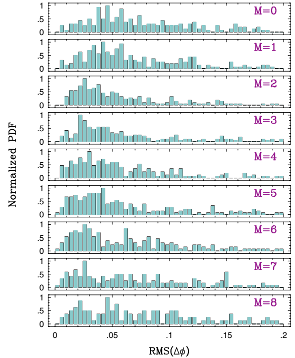
Fig. 2. Probability distribution functions of the average phase differences \text{rms}(\Delta\varphi) (Eq. (3)) for test targets at various template polynomial degrees M . All target light curves were generated with N = 20 data points. No noise is added. The test was performed on the basic data set. Each PDF is normalized to its maximum. We draw attention to the narrowing of the PDFs at low M values of 2–4.
