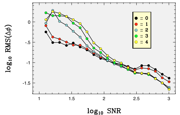
Fig. 5. Dependence of the average of \text{rms}(\Delta\phi) on SNR at various template polynomial degrees M shown in the inset. The figure is based on simulated data described in detail in the text.
