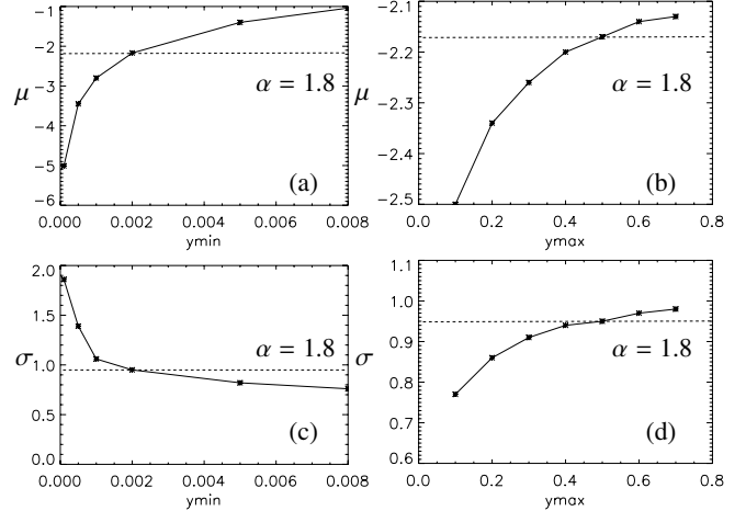
Fig. 5. Variation of the lognormal scale and shape parameters with the lower a ), c ) and upper b ), d ) cutoffs of the flare amplitude distribution. The values employed for the other parameters are \alpha = 1.8 , \tau_d = 8.01 , p_f = 0.60 , ( y_{\min} variable, y_{\max} = 0.5 ); and ( y_{\max} variable, y_{\min} = 0.002 ). The horizontal dashed lines represent observed values (averages over O IV quiet network area).
