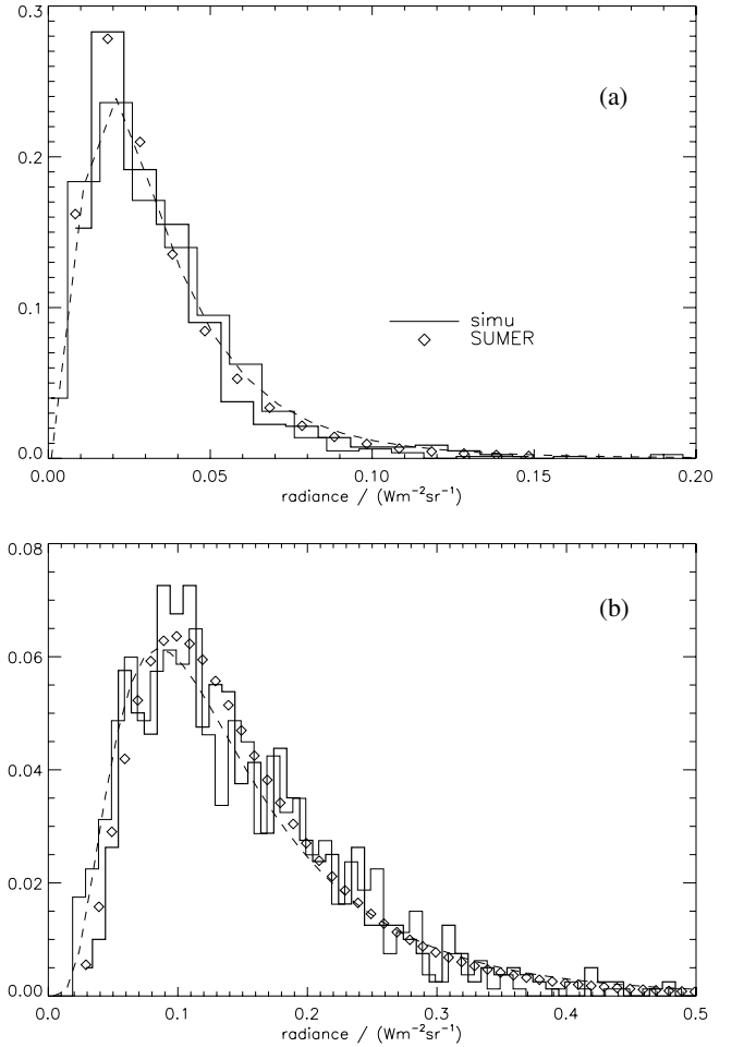
Fig. 11. Histograms and lognormal fits of the simulated (thin-line histogram and dashed curves, respectively) and SUMER (O IV line at 79.0 nm) measured (thick-line histogram and diamonds) radiances. a) from a time series in a very quiet area (cell interior), b) from a network sample of the same size ( 1'' \times 1'' ).
