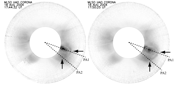
Fig. 1. Vignettted MK4 negative images of the CME on 2004 August 18. The MK4 field of view is from 1.08 to 2.85 R_{\odot} . Arrows indicate the CME heights measured along two dotted lines of the CME nose (PA1 = 250°) and CME flank (PA2 = 230°) near the helmet streamer, respectively.
