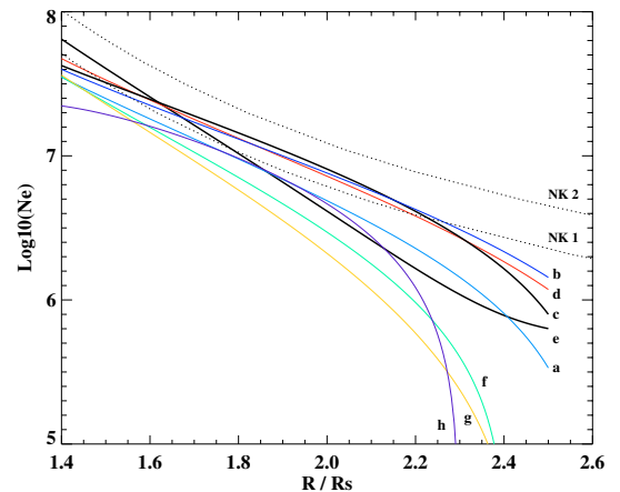
Fig. 4. Measured coronal density distributions along the position angles denoted in Fig. 3. The distributions at the northern flank of the CME at 276° (g) and 282° (g') are similar to each other. Dotted lines denoted as NK1 and NK2 represent the one- and two-fold Newkirk density models, respectively.
