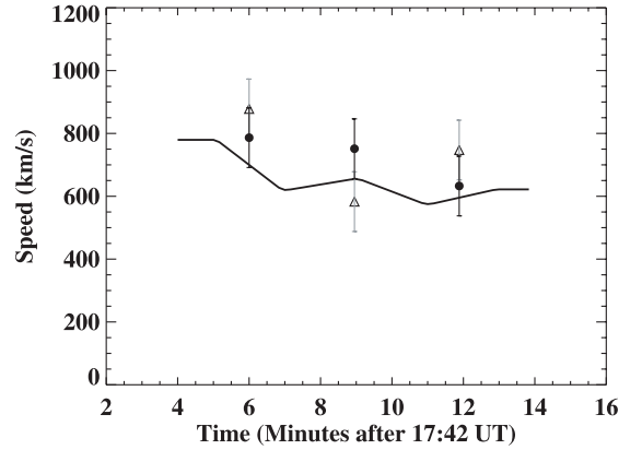
Fig. 6. Speed comparison among coronal shock (solid line) estimated density profile (c) along southern CME flank, CME front (triangles), southern CME flank (filled circles). The error bars indicate the uncertainty ( \pm 95 \text{ km s}^{-1} ) of CME speed due to measurement errors (2-pixels) in MK 4 image.
