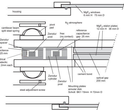
Fig. 14. Schematic of the piezoelectric-tunable, capacitance-stabilized VUV FP etalon. Each piezoelectric driver is matched with a capacitor made of metallized Zerodur post providing electronic tuning of the optical gap. The \text{MgF}_2 etalon plates are cemented to mounting plates that are held by a Hansen cantilever beam. The \text{MgF}_2 housing window holds a pure \text{N}_2 atmosphere for transmittance at 155 nm. The reflectance \Pi -coatings cover 30 mm area centered on the etalons. The annular holes in the glass mounting plates are 35 mm diameter.
