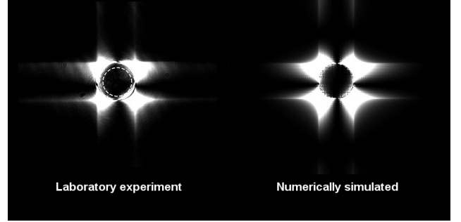
Fig. 2. Coronagraphic pupil images. Left: laboratory experiment. The dashed circle represents the Lyot stop that is used for on-sky observations (see Sect. 4.2). Right: numerically simulated. We introduced suspected phase-shift defects to simulate the pupil intensity distribution (thresholded images to exhibit the intensity distribution structures).
