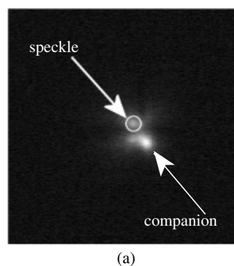
Fig. 7. On-sky data of HD 80081. a) Without the coronagraph (monitoring camera); b) with the coronagraph (science camera). This image was obtained by co-adding 126 frames selected among the 5000 recorded frames, using the selection algorithm described in Sect. 6.2. The companion appears clearly in the coronagraphic image.
