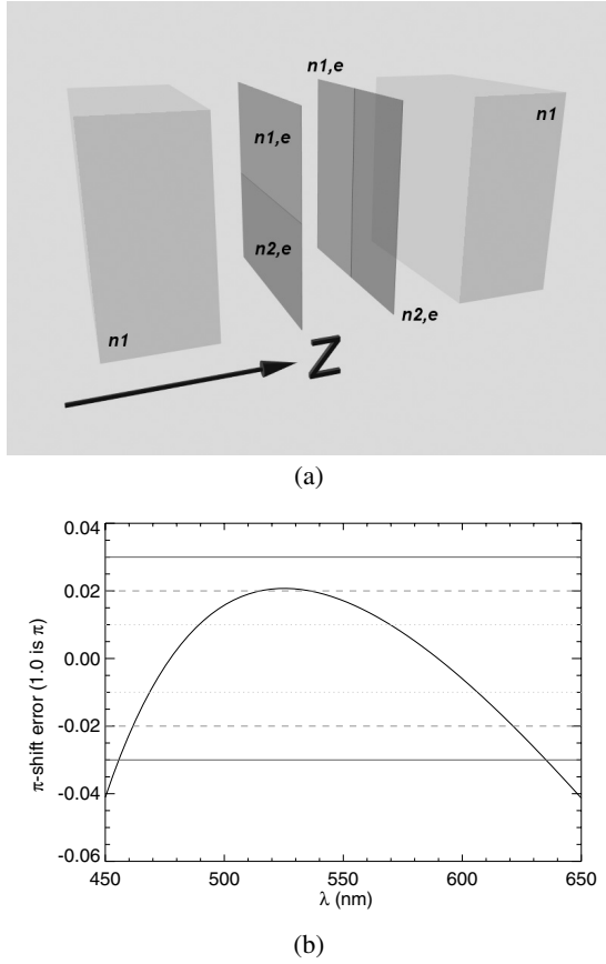
Fig. 1. a) The optical assembly of the APKC component: two 99\ \mu\text{m} phase knives are stacked between two 6 mm thick glass plates. The light propagates along the Z axis. b) The relative error on the \pi phase-shift over the considered spectral bandwidth.
