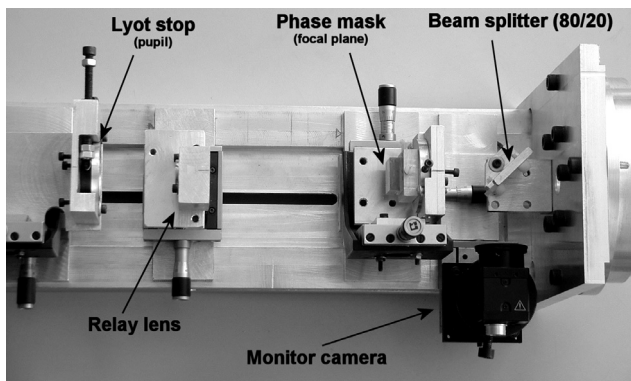
Fig. 6. Coronagraphic optical bench (see text for details). The refractor's bonnet is out of frame on the right side, and the science camera is out of frame on the left side. The light propagates from right to left.
