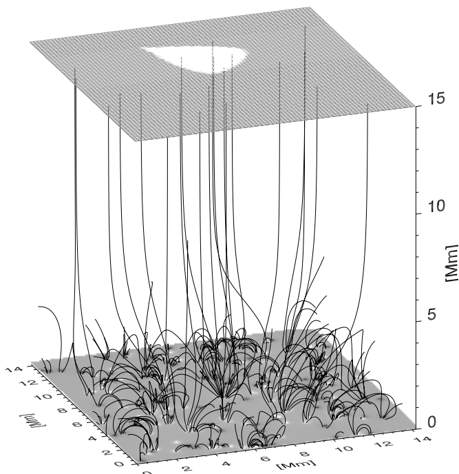
Fig. 1. Composite plot of the magnetic field at the bottom (lower BC), field lines of the extrapolated magnetic field, and a mask of the area at 15 Mm height that is magnetically connected to the central strong network magnetic patch (white).
