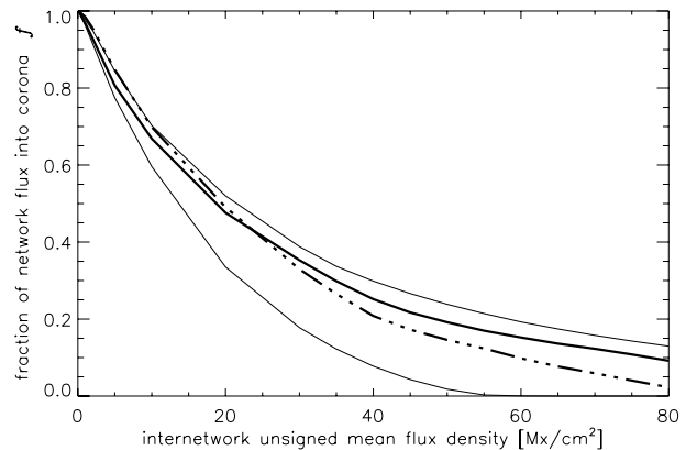
Fig. 2. Average fraction f of magnetic flux from the strong network patch into the corona as defined in (6) as a function of the unsigned mean internetwork flux density. The dot-dashed line shows the result for a point charge model similar to Schrijver & Title (2003), see Sect. 3.1. The thick solid line displays f for the field extrapolation using a Fourier transform technique. For all (!) of the four upper boundary conditions discussed in Sect. 2.2.2 the results are practically the same. While the thick line represents the median value of f for the different spatial random distributions of internetwork patches, the thin lines show the scatter (enclosing 2/3 of all values for f ). See Sects. 3.1 and 3.2.
