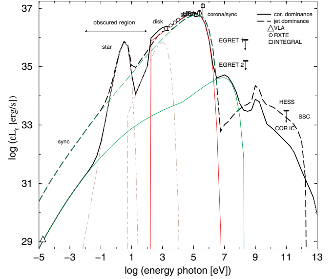
Fig. 1. Computed broadband SED for 1E 1740.7–2942 for a dominant X-ray corona (thick solid line) and a dominant X-ray jet (thick long-dashed line) (see Table 2). Data points and observational upper-limits are also shown. Note that radio constraints are violated for the dominant X-ray jet case. We note that dips at \sim 100 MeV and few GeV are due to photon-photon absorption in the corona and the disk photon fields respectively. At the radio band, the core luminosity at the adopted distance is shown. The slope at this range is similar to that observed (not shown explicitly; see Fender 2001, and references therein). At X-rays/soft gamma-rays, RXTE and INTEGRAL data are plotted (Del Santo et al. 2005). At high-energy gamma-rays, two upper-limits are shown: one from the spectrum of the source 3EG J1744–3011 (EGRET 1), as absolute upper-limit (Hartman et al. 1999), and the other obtained from the sensitivity limits of EGRET (EGRET 2) in the region (Hartman et al. 1999). The diffuse emission flux at \geq 100 GeV observed by HESS in the direction of the source is shown as an upper-limit (Aharonian et al. 2006).
