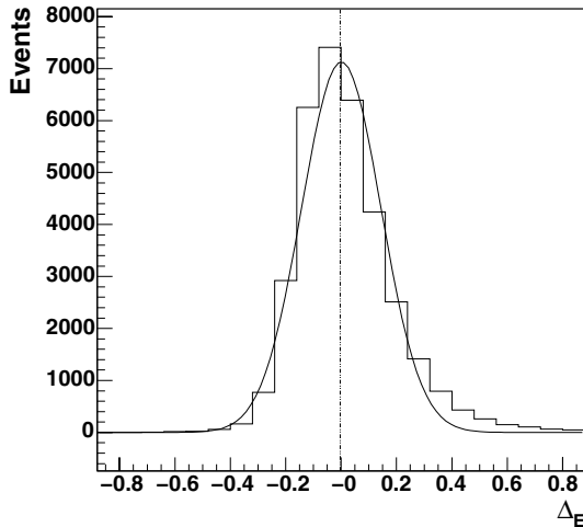
Fig. 12. The distribution of the relative error in the reconstructed energy per event for Monte Carlo simulated \gamma -rays with a power law energy distribution (above 440 GeV) with \Gamma = 2.6 at 50^\circ zenith angle. The root mean square (rms) width of this distribution is 16%. The width of the fitted Gaussian distribution is 14%.
