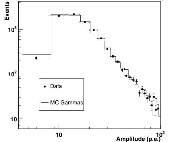
Fig. 3. Distribution of the intensity of the 3rd highest pixel for 4 telescopes (points), compared with Monte Carlo simulations (solid lines). The overall flux of the simulated data has been adjusted to fit the real data.
