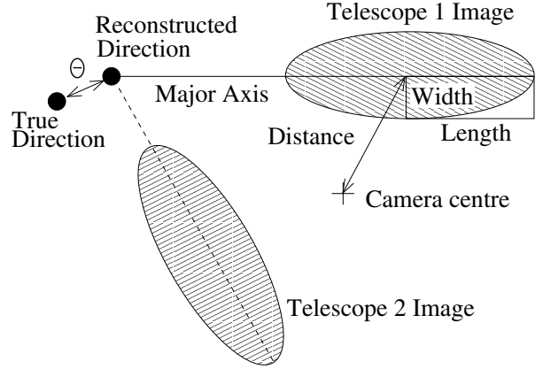
Fig. 5. Definition of simple Hillas parameters, calculated for a \gamma -ray image, which may be approximated as an ellipse. Important parameters for this analysis are the width, length, distance. An image from a second telescope is superimposed to demonstrate the geometrical technique for source position reconstruction. The parameter \theta , which is the magnitude of the angular offset in shower direction reconstruction, is also shown.
