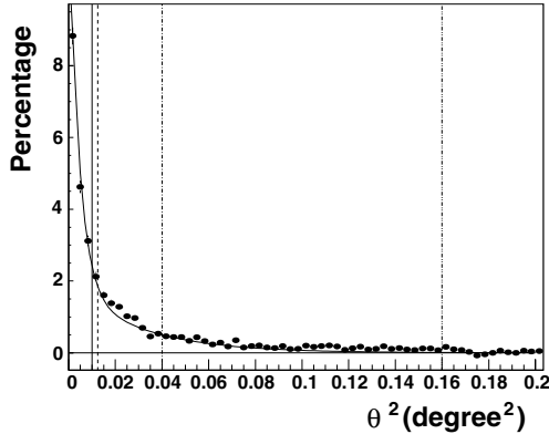
Fig. 6. Distribution of excess events in \theta^2 for the complete Crab data set, after event selection and background subtraction. The Monte Carlo derived point-spread function described in Eq. (1) is also shown, normalised to the excess distribution. The vertical lines denote the \theta^2 selection cuts listed in Table 2.
