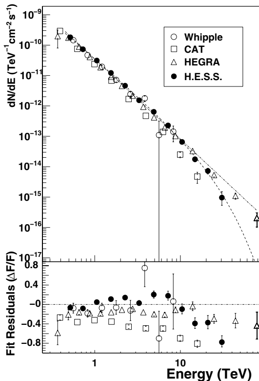
Fig. 20. Comparison between the spectral measurements of CAT (open squares), Whipple (open circles) and HEGRA (open triangles) and the results of this study (filled circles). The residuals are shown for each spectrum relative to a power law fit to the HESS data (dotted line).
