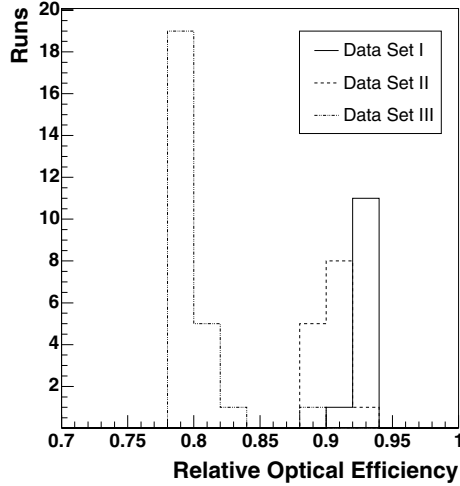
Fig. 4. Distribution of the relative optical efficiency per run for data sets I (solid line), II (dashed line) and III (dotted line). It can be seen that the relative optical efficiency is significantly decreased in data set III relative to the other data sets.
