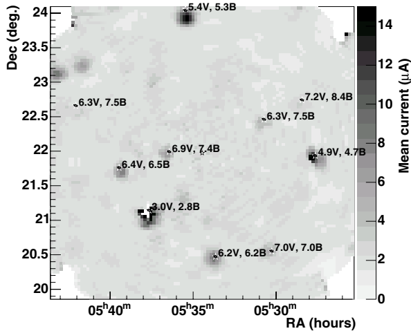
Fig. 2. Sky map of DC pixel current (in units of \mu\text{A} , measured in a window of 16 \mu\text{s} ) for the region surrounding the Crab nebula. The positions of stars (read from the Hipparcos catalogue – Perryman & ESA 1997) match well with the peaks in the map, which correspond to peaks in sky brightness. The B and V magnitudes of each star are also given for comparison. The brightest star, \zeta Tauri ( B magnitude 2.8), has caused the camera to disable PMTs, thus there is no current measure for the region close to this star.
