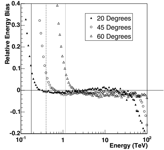
Fig. 11. Relative bias ((E_{\text{reco}} - E_{\text{true}}) / E_{\text{true}}) in estimation of energy as a function of energy for three zenith angles. The vertical lines represent the safe energy thresholds for spectral analysis at each zenith angle.
