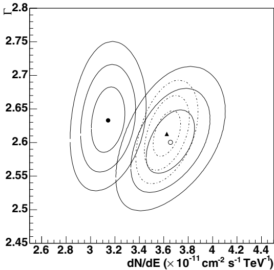
Fig. 19. Contour plot of the \chi^2 fit error as a function of the power law parameters F_0 and \Gamma for data sets I (filled circle), II (open circle) and III (filled triangle, dotted lines). The 68%, 95% 99.9% error contours are shown, and The best fit spectral parameters are marked in each case.
