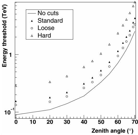
Fig. 14. The peak-rate energy threshold before and after selection cuts versus zenith angle, for three sets of selection cuts as described in Table 2. The safe threshold for spectral analysis in each case is slightly higher.
