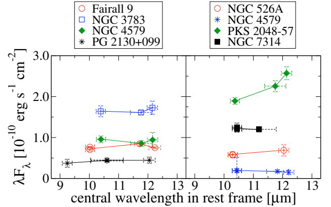
Fig. 1. The MIR SEDs of our sample of galaxies. Early- and late-type Seyferts are shown in the left- and right-hand panel respectively. Horizontal error bars show the band width of the used filters. The flux densities of NGC 7314 have been offset by +1 \times 10^{-10} \text{ erg s}^{-1} \text{ cm}^{-2} for clarity.
