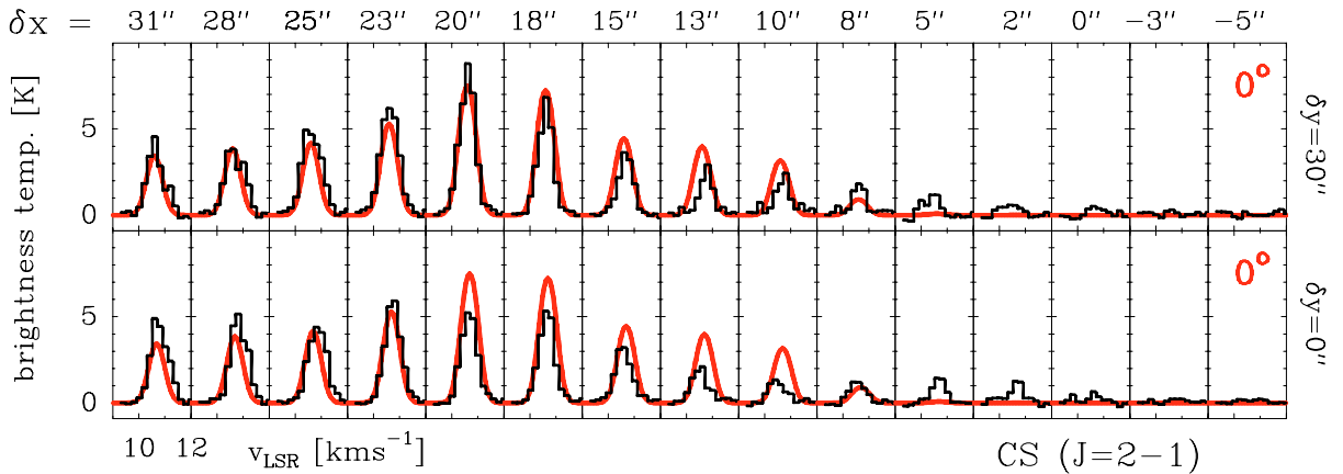
Fig. 11. IRAM-PdBI CS J = 2-1 spectra along the direction of the exciting star at \delta y = 30'' ( upper panel ) and \delta y = 0'' ( lower panel ). Radiative transfer models using the output of PDR models for CS (red curve) for a density gradient and physical conditions discussed in the text (assuming that the PDR is not inclined relative to the line of sight). Modeled line profiles have been convolved with an appropriate Gaussian beam corresponding to each synthesized beam. Intensity scale is in brightness temperature and abscissa in LSR velocity.
