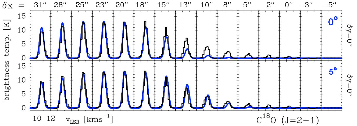
Fig. 10. IRAM-PdBI C^{18}O J = 2-1 spectra along the direction of the exciting star at \delta y = 0'' (histograms). Radiative transfer models using the output of PDR models for C^{18}O (blue curve) for a density gradient and physical conditions discussed in the text. Lower panel shows inclination effects assuming that the PDR is inclined relative to the line of sight by a \varphi = 5^\circ angle. Modeled line profiles have been convolved with an appropriate Gaussian beam corresponding to each synthesized beam. Intensity scale is in brightness temperature and abscissa in LSR velocity.
