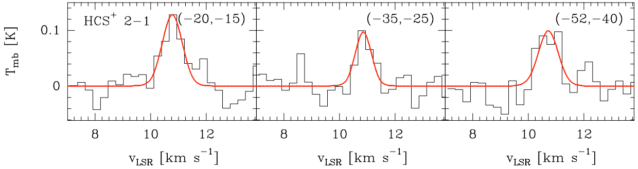
Fig. 8. IRAM-30 m \text{HCS}^+(2-1) single-dish observations (histograms) at different positions of the Horsehead. Offsets in arcsec refer to the (0,0) position of the \text{C}^{18}\text{O}(2-1) map (see Fig. 4). Radiative transfer models for \text{HCS}^+ at selected positions are also shown (curves). Predicted line profiles have been convolved with the telescope angular resolution at each frequency. Intensity scale is in main beam temperature.
