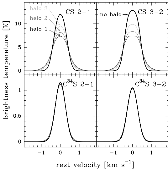
Fig. 13. CS and C^{34}S synthetic line profiles for a cloud with a depth of 0.1 pc, T_k = 30 K, n(H_2) = 10^5 cm ^{-3} and \chi(CS) = 7 \times 10^{-9} (thick curves). Thin curves show the resulting spectra if the same cloud is surrounded by different diffuse halos (3: n(H_2) = 5 \times 10^3 cm ^{-3} , 2: n(H_2) = 8 \times 10^3 cm ^{-3} and 1: n(H_2) = 1 \times 10^4 cm ^{-3} ). The CS abundance in the cloud is determined more precisely from CS high- J and C^{34}S low- J observations, otherwise it is underestimated. Note that the intensity levels are comparable to those observed in the Horsehead.
