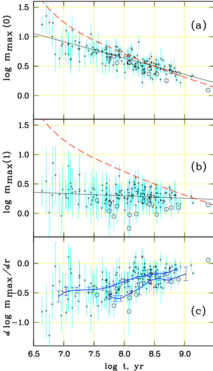
Fig. 12. The expected mass of the brightest stars computed for the cluster centres a ) and edges b ) versus cluster age. Panel c ) shows the variation of radial mass gradient d \log m_{\max}/dr with cluster age. Circles indicate all clusters included in the analysis, large open circles mark the subsample of nearby clusters ( (V - M_V) < 7.3 ) with the most extended Main Sequences. The rms errors of the individual data points are shown as light grey (cyan) bars. In panels a ) and b ) the dashed curves show the “mass–MS–lifetime relation” based on the Padova isochrones with overshooting for Z = 0.019 , solid lines present the solution of Eqs. (4), (5). In panel c ) the curves show the running average of the radial mass gradient computed with a (\log t) -bin of 0.6 and a step of 0.2 for nearby clusters (lower curve) and for all other clusters (upper curve). The rms errors of the corresponding averages are shown with bars.
