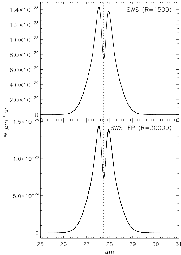
Fig. 4. Same as Fig. 3 for the naphthalene band at 27.74 \mu\text{m} . The rotational constants are almost unchanged in the vibrational transition, resulting in a very symmetric rotational envelope, the asymmetry being mainly due to the superposition of slightly displaced sovratones of the band.
