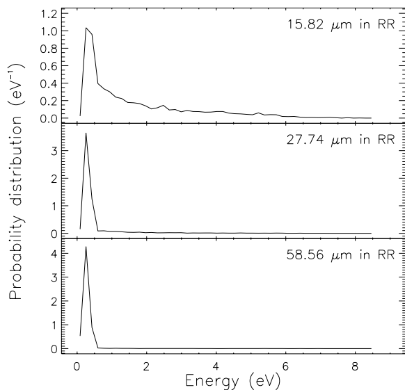
Fig. 1. Probability distribution of the excitation energies at which photons are emitted in the three bands of neutral naphthalene considered, in the Red Rectangle halo.
