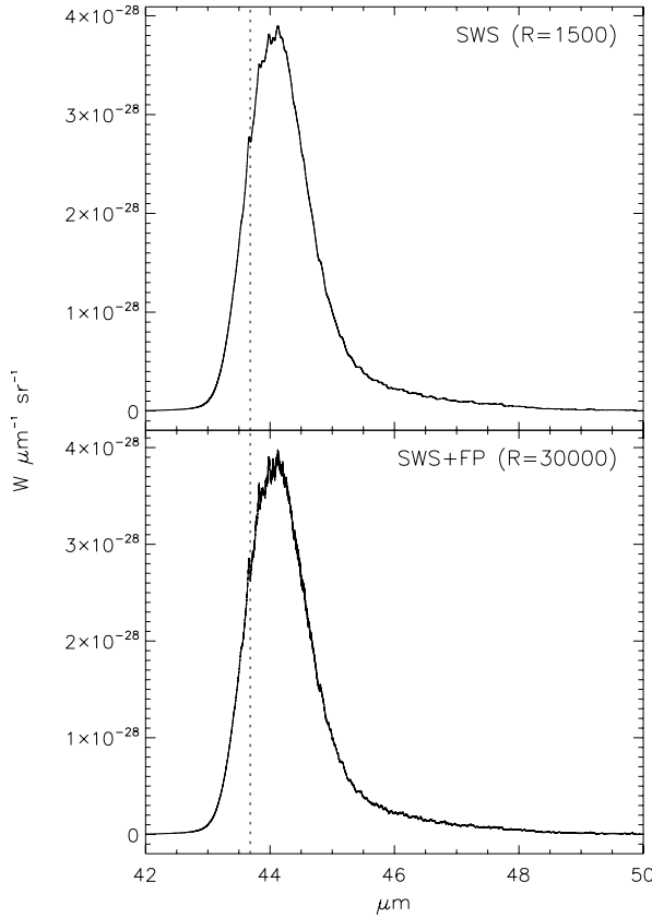
Fig. 8. Same as Fig. 6 for the anthracene band at 43.68 \mu\text{m} . The relatively large change in the rotational constants in the vibrational transition results in a visibly red-shaded band.
