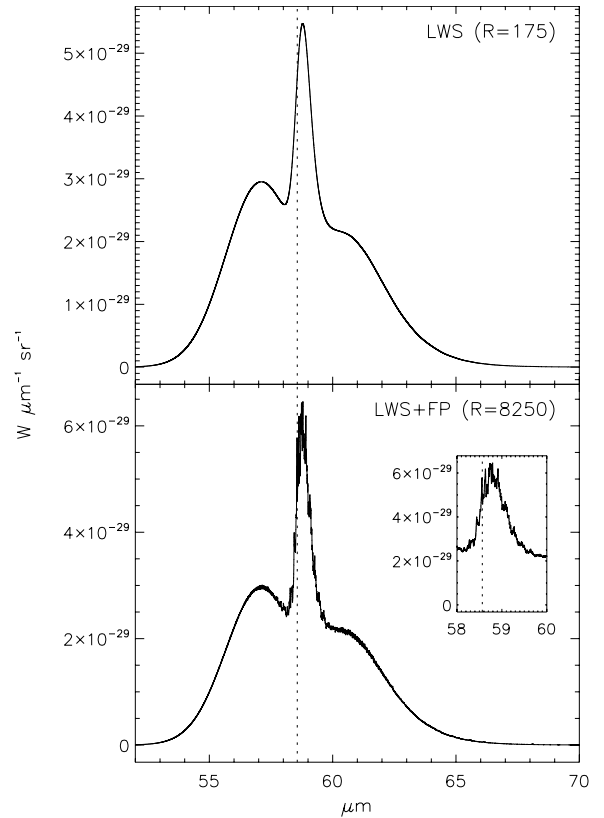
Fig. 5. Same as Fig. 3 for the naphthalene band at 58.56 \mu\text{m} . The rotational constants are almost unchanged in the vibrational transition, resulting in a relatively symmetric rotational envelope, with a Q branch standing out very clearly. The two panels show the band as it would be seen by ISO-LWS, with and without the Fabry-Perot filter. In the lower panel, the higher resolving power allows the resolution, in the Q branch, of the separate contributions of different hot bands, with slightly different anharmonic shifts (zoomed inset).
