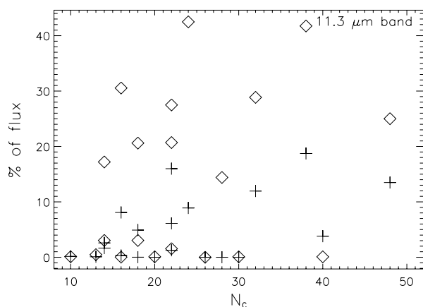
Fig. 13. Same as Fig. 11 for the out-of-plane C-H bend at \sim 11.3 \mu\text{m} . Here, for each molecule, we considered all bands in the range 10.9 to 11.7 \mu\text{m} , which corresponds to the observed width of the 11.3 \mu\text{m} band in the Red Rectangle.
