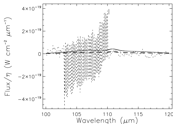
Fig. 10. Comparison between the estimated IR emission spectrum of anthracene ( \text{C}_{14}\text{H}_{10} ) and an ISO spectrum of the Red Rectangle in the wavelength range 100–120 \mu\text{m} . Calculated spectra, under different assumptions (see Mulas et al. 2006b, for details), are drawn in dashed, dash-dotted, and continuous lines; the continuum-subtracted ISO spectrum is shown as a dotted line. The central position of the fundamental of the expected anthracene band is marked by a tick, which shows the effect of anharmonic shifts.
