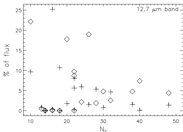
Fig. 12. Same as Fig. 11 for the out-of-plane C-H bend at \sim 12.7 \mu\text{m} . Here, for each molecule, we considered all bands in the range 12.3 to 13.1 \mu\text{m} , which corresponds to the observed width of the 12.7 \mu\text{m} band in the Red Rectangle.
