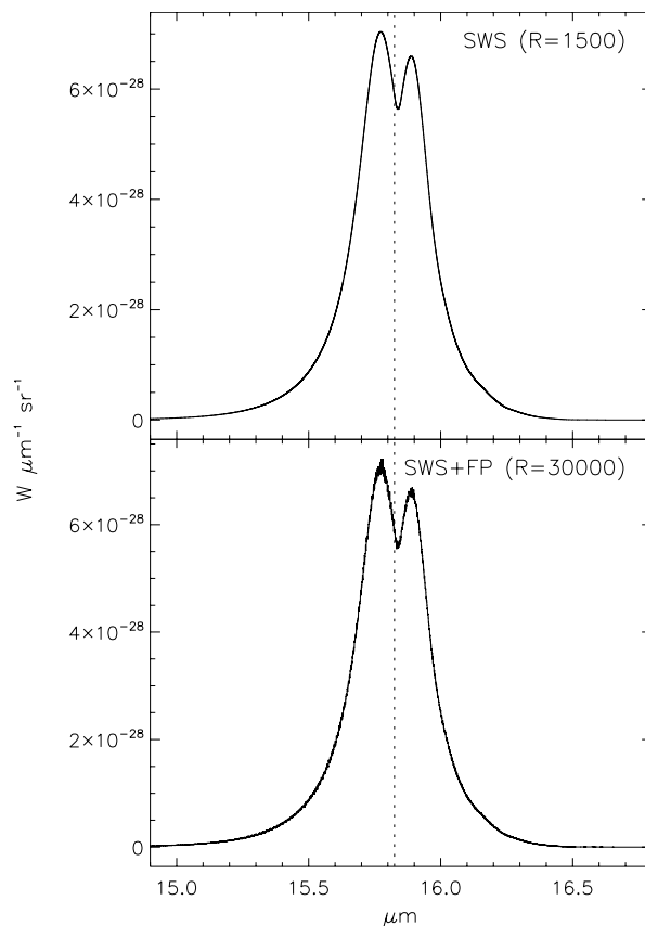
Fig. 3. Detailed rotational structure of the band of neutral naphthalene at 15.82 \mu\text{m} in the Red Rectangle halo. Strong Coriolis coupling with the IR-inactive band at 15.90 \mu\text{m} causes one of the rotational constants to differ by \sim 4\% between the upper and lower vibrational states involved in the transition, producing a blue shaded rotational profile. The superposition of hot bands, which has a red-shaded envelope, acts in the opposite direction, so that the overall profile including both effects is almost symmetric. The two panels show the band as it would be seen by ISO-SWS with and without the Fabry-Perot filter. The vertical dotted line marks the position of the origin of the fundamental band.
