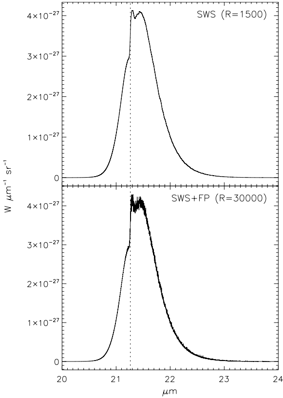
Fig. 6. Detailed rotational structure of the band at 21.26 \mu\text{m} of neutral anthracene in the Red Rectangle halo. The rotational constants are almost unchanged in the vibrational transition, resulting in a very symmetric rotational envelope, with a visible Q branch whose width is due to the superposition of hot bands with different anharmonic shifts. The two panels show the band as it would be seen by ISO-SWS, with and without the Fabry-Perot filter. The vertical dotted lines marks the position of the origin of the fundamental band.
