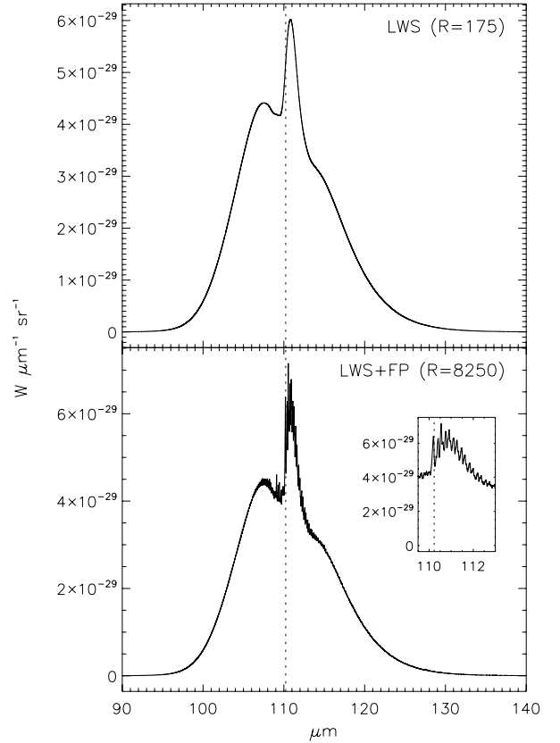
Fig. 9. Same as Fig. 6 for the anthracene band at 110.23 \mu\text{m} . The change in rotational constants, combined with the superposition of hot bands, produces an asymmetric profile, in the middle of which a sharp Q branch clearly stands out. In the lower panel, the higher resolving power allows the resolution, in the Q branch, of the separate contributions of different hot bands, with slightly different anharmonic shifts (zoomed inset).
