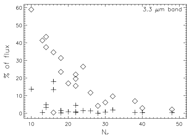
Fig. 11. Percentage of total IR flux emitted in the in-plane C-H stretch near \sim 3.3 \mu\text{m} , as computed by our model for the sample of molecules in Mulas et al. (2006a), shown as a function of molecular size. Neutral species are represented by diamonds, cations by crosses. Here, for each molecule, we considered all bands in the range 3.2 to 3.37 \mu\text{m} , which corresponds to the observed width of the 3.3 \mu\text{m} band in the Red Rectangle.
