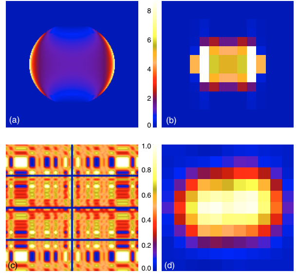
Fig. 3. a) The expected image at 28 keV (in units of 10^{-26} erg \text{cm}^{-2} \text{s}^{-1} \text{Hz}^{-1} \text{sr}^{-1} ) based on simulations performed by Reynolds (1999). b) The sampled sky image in the ISGRI sky pixels size (in units of \text{ct s}^{-1} ). c) The corresponding shadowgram of the PIF values and d) the reconstructed image after the standard deconvolution (in units of \text{ct s}^{-1} ).
