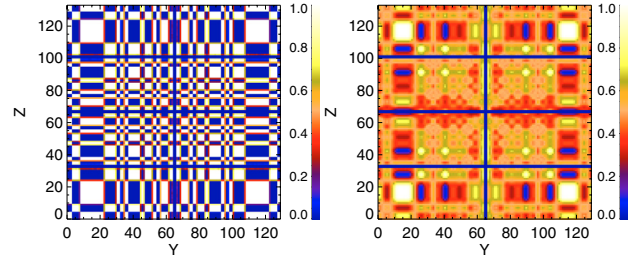
Fig. 1. The recorded ISGRI shadowgram of the PIF values for an on-axis point-like source (left) and that of a uniform disk of \sim 20' radius (right) without background. Dead zones between modules and mask elements are clearly visible.
