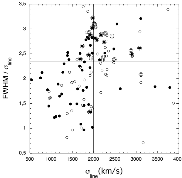
Fig. 3. The H \beta line-width ratio FWHM/\sigma_{\text{line}} versus \sigma_{\text{line}} in all the datasets in Table 1. The open and filled circles correspond respectively to values based on mean and rms spectra. The large symbols mark the different datasets for NGC 5548. The horizontal line is the value of the ratio for a Gaussian profile, and the vertical line is an arbitrary division at \sigma_{\text{line}} = 2000 \text{ km s}^{-1} . The horizontal line divides the samples into our Populations 1 ( lower ) and 2 ( upper ), and the vertical line approximates the division of Sulentic et al. (2000) into Populations A ( left ) and B ( right ).
