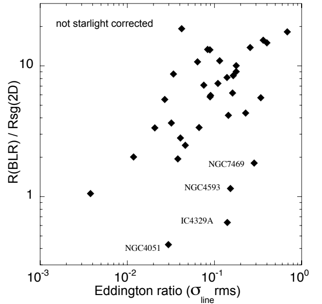
Fig. 11. The ratio R_{BLR}/R_{sg} , as described in the text. The four outliers are objects whose luminosity and Eddington ratio are probably overestimated (see the text). If R_{BLR}/R_{sg} > 4 , the BLR is gravitationally unstable.
