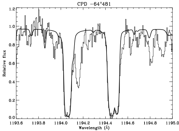
Fig. 5. The S III resonance lines for CPD -64^{\circ}481 , showing an excellent match. The line at \sim 1194.5 \text{ \AA} is one of the Si II resonance lines, while the strong line at \sim 1194.15 \text{ \AA} is unidentified.
