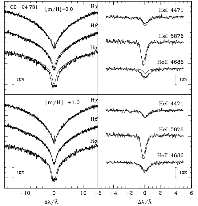
Fig. 2. Same as Fig. 1 but for CD -24^{\circ}731 .
