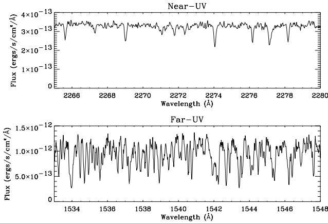
Fig. 3. Comparison of a 15 Å wide section of the near- and far-UV spectrum of PG 1219+534. In the NUV it is possible to measure the continuum level, while in the FUV it must be estimated. Note also the higher flux in the FUV.
