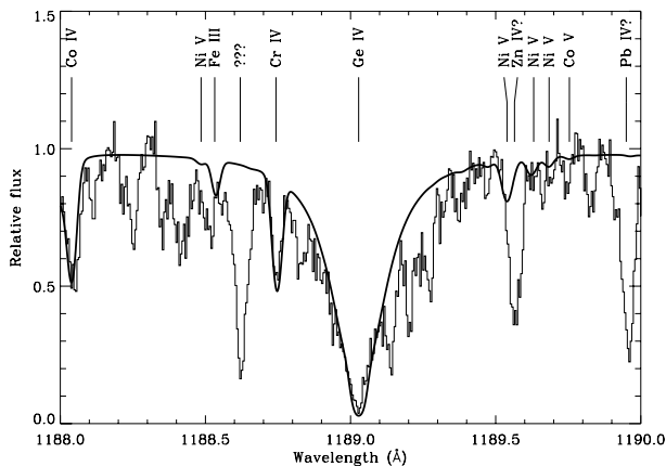
Fig. 10. Spectrum fit to the Ge IV resonance lines at 1189 Å for Feige 66. The model is shown as the thick line.
