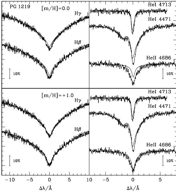
Fig. 1. Line profile fit for PG 1219+534 using solar metallicity models ( top panel ) and metal-rich models (10 times solar, bottom panels ). The Balmer lines and He II at 4686 Å match simultaneously when using the metal rich models (see text).
