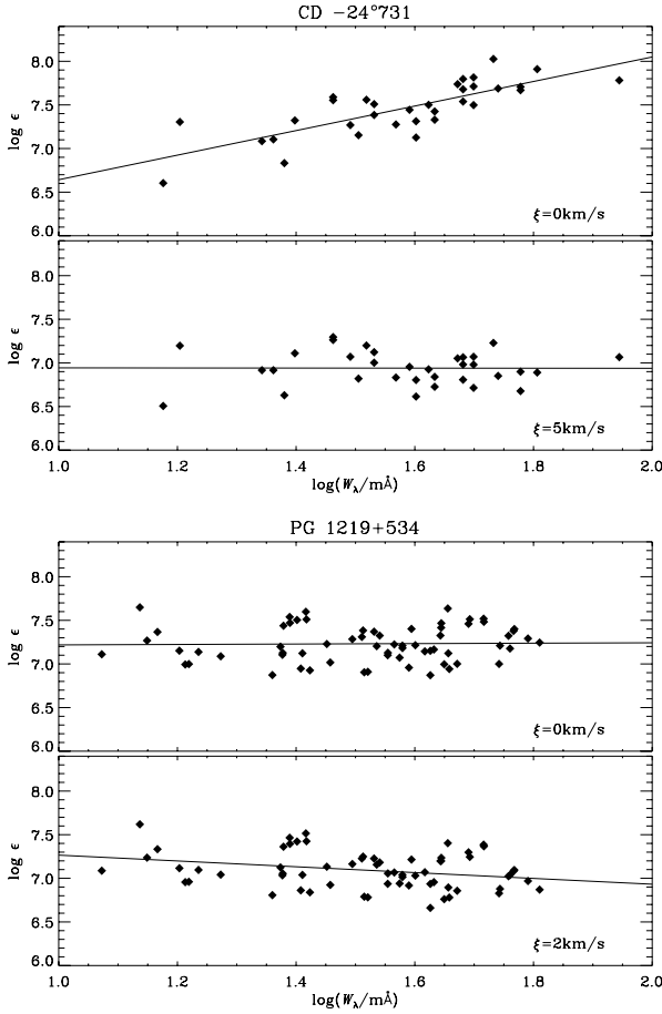
Fig. 7. Determination of microturbulent velocity of CD -24^{\circ}731 and PG 1219+534 using Cr III lines. We find \xi = 5^{+2}_{-1} km s ^{-1} for the former, while the latter is consistent with \xi = 0 km s ^{-1} .
