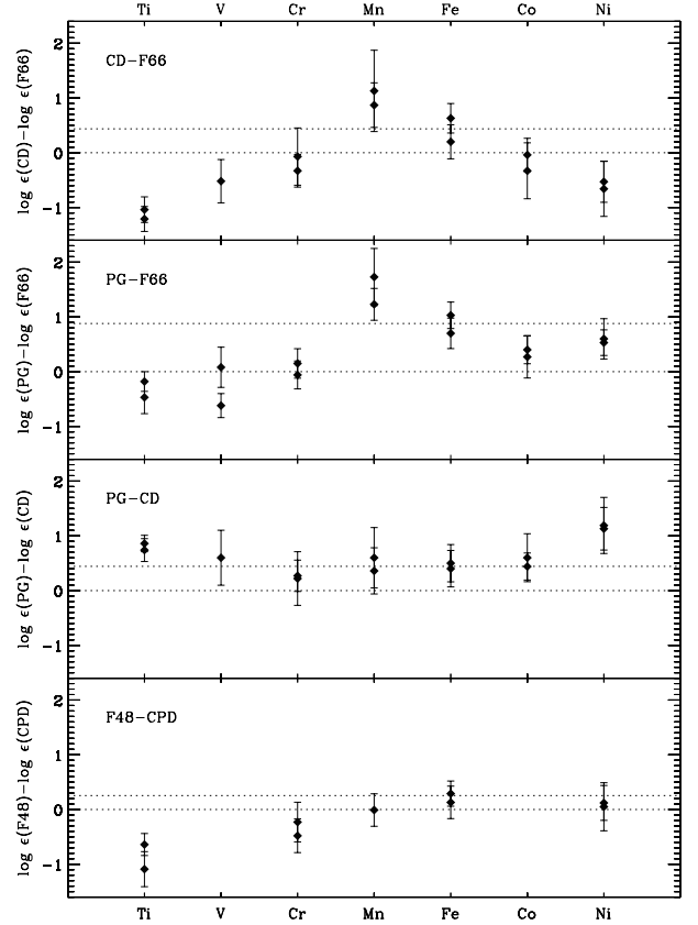
Fig. 12. Comparison of iron-group abundances for our pulsator/non-pulsator pairs (F48 = Feige 48; CPD = CPD -64^{\circ}481 ; PG = PG 1219+534; CD = CD -24^{\circ}731 ; F66 = Feige 66). The dotted lines denote equal abundances and the difference in iron abundance. The differences between PG 1219+534, CD -24^{\circ}731 and Feige 66 are quite large – particularly for Fe, Ni and Mn – while the pairs PG 1219+534 and CD -24^{\circ}731 and Feige 48 and CPD -64^{\circ}481 show quite similar abundances, in particular when the differences in iron abundance are accounted for (see text).
