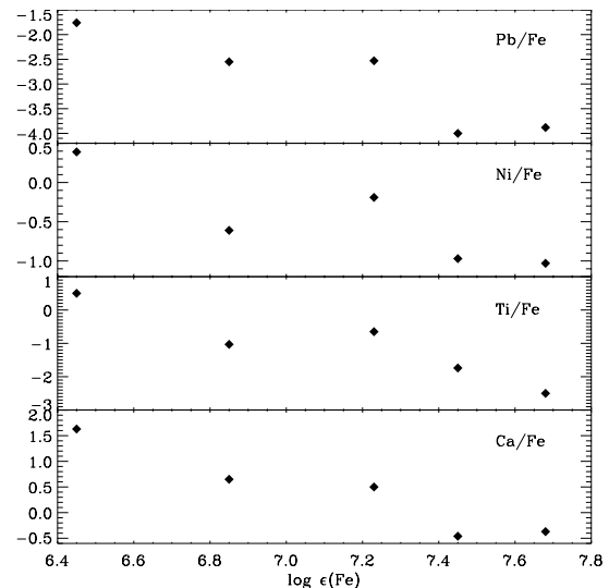
Fig. 11. Trends in heavy element abundances with iron abundance.
