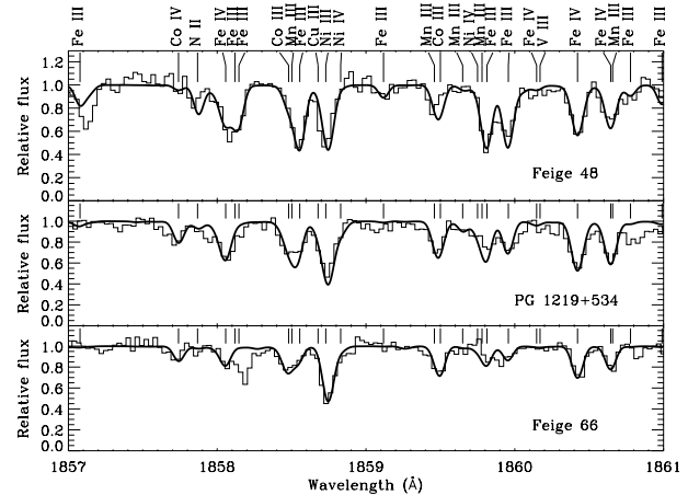
Fig. 6. A region of spectrum showing blended iron-group lines for Feige 48, PG 1219+534 and Feige 66. The line at \sim 1858.2 \text{ \AA} is unidentified.
