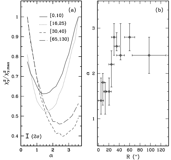
Fig. 7. The CMD method for NGC 1831. Panel a ) illustrates how the statistic \chi^2_\gamma varies with the adopted \alpha used in the CMD models at different concentric annuli. Panel b ) shows the best-fit \alpha vs. R relation.
