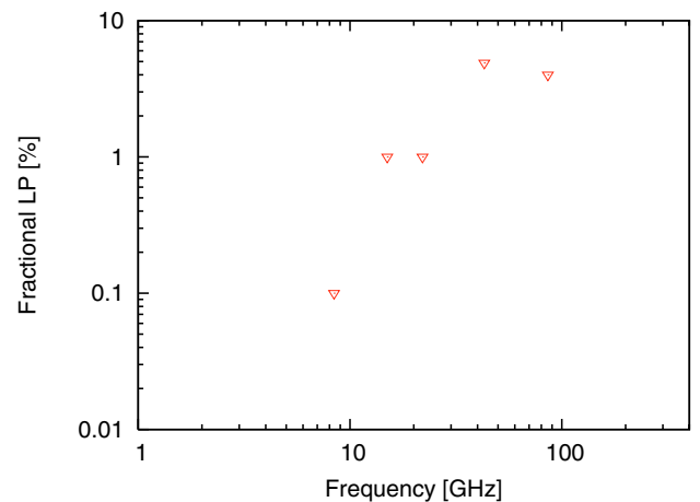
Fig. 5. 3\sigma upper limits on the linear polarization of M 81* up to 86 GHz. The 8.4 GHz data point is taken from Bower et al. (2002a).
