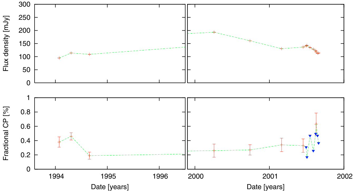
Fig. 1. Light-curve in total intensity ( top ) and fractional circular polarization of M 81* at 4.8 GHz for the archival data ( left ) and the new observations ( right ). The filled triangles are 3\sigma upper limits. The two data points in 2000 are taken from Brunthaler et al. (2001).
