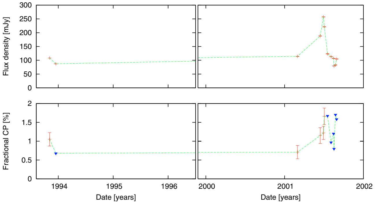
Fig. 3. Light-curve in total intensity ( top ) and fractional circular polarization of M 81* at 15 GHz for the archival data ( left ) and the new observations ( right ). The filled triangles are 3\sigma upper limits.
