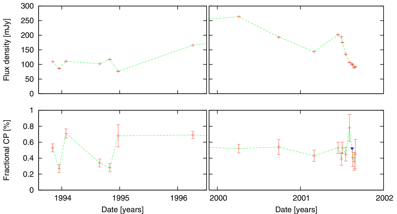
Fig. 2. Light-curve in total intensity ( top ) and fractional circular polarization of M 81* at 8.4 GHz for the archival data ( left ) and the new observations ( right ). The filled triangle is an 3\sigma upper limit. The two data points in 2000 are taken from Brunthaler et al. (2001).
