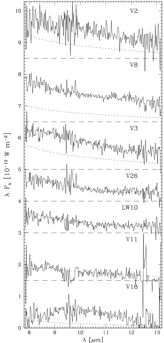
Fig. 2. The 8–13 \mu\text{m} spectra for the other targets in 47 Tuc, in order (from bottom to top) of increasing 8.6 \mu\text{m} brightness. The dashed line indicates the zero-level for each spectrum. The dotted curve is the template spectrum for M3.5 V star \gamma Crux scaled to match the 2.2 \mu\text{m} flux density of the target star.
