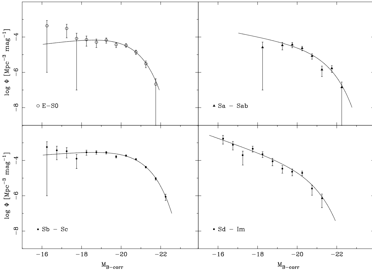
Fig. 7. OLF for the different morphological types present in the CIG sample together with the corresponding Schechter fit shown as a solid line.
