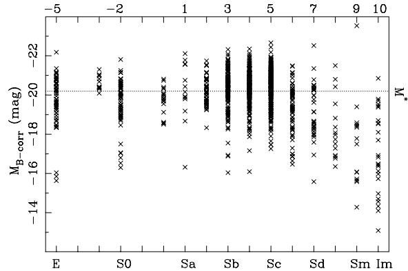
Fig. 3. Distributions of new morphologies as a function of absolute magnitude M_{B\text{-corr}} . The abscissa indicates basic Hubble subtypes (bottom) and corresponding RC3 numeral types (top). The dotted line shows the total sample M^* derived in Paper I.
