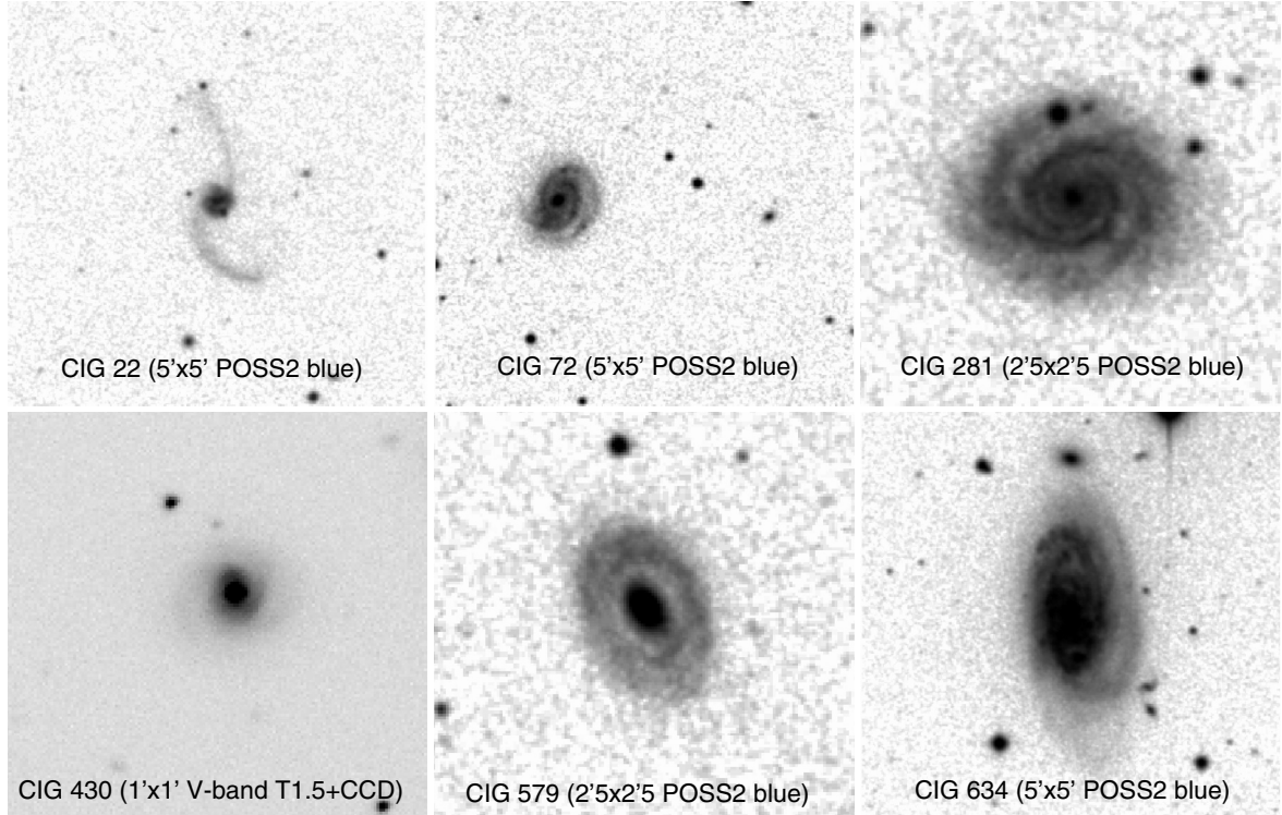
Fig. 1. Six examples of CIG galaxies from POSS II images unless otherwise noted. Upper left: CIG 22, classified I/A = y, shows “integral sign” structure almost certainly due to interaction although a companion cannot yet be identified. Upper centre: CIG 72, an Sc spiral showing both disk distortion and an active nucleus with a likely dwarf companion. Upper right: CIG 281, a prototype isolated Sc spiral. Lower left: for CIG 430, the OSN CCD images (stack of 3 \times 900 s exposures in V shown here, seeing 1''.4 ) reveal faint spiral arms in a CIG often previously classified as early-type. Lower centre: CIG 579, a rare prototype isolated galaxy with a large bulge, classified as Sab. Lower right: CIG 634, classified I/A = y showing morphological distortion and a LINER nucleus; dwarf companion visible on the northern edge.
