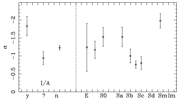
Fig. 9. The same as in Fig. 8 for the \alpha parameter.
