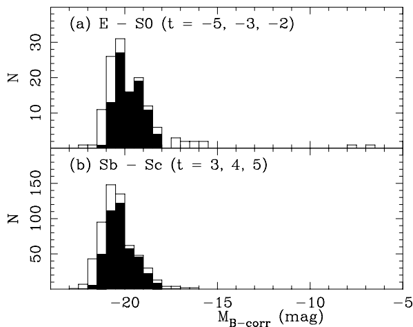
Fig. 5. Luminosity distribution for the indicated populations both for the complete sample and (solid) for galaxies in the range V_R = 2000\text{--}10\,000 km s -1 .
