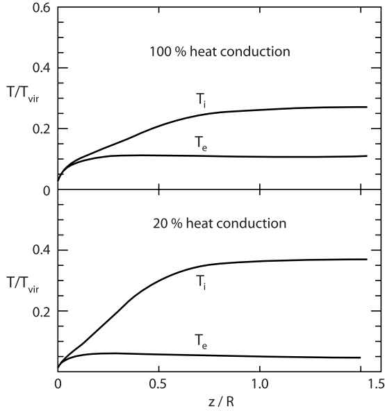
Fig. 2. Coronal temperatures: electron and ion temperatures (measured in virial temperature) at height z/R , R distance from black hole, z height above midplane.
