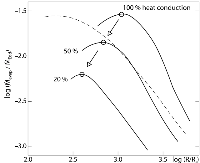
Fig. 1. Effect of reduced heat conduction: evaporation rate as a function of distance from the black hole (hard spectral state). Solid lines: thermal conduction according to standard Spitzer rate and reduced to 50% and 20%. Dashed line: 100% heat conduction, but without irradiation. Reduced heat conduction leads to disk truncation farther inward. The maxima give locations of innermost disk truncation at spectral transition.
