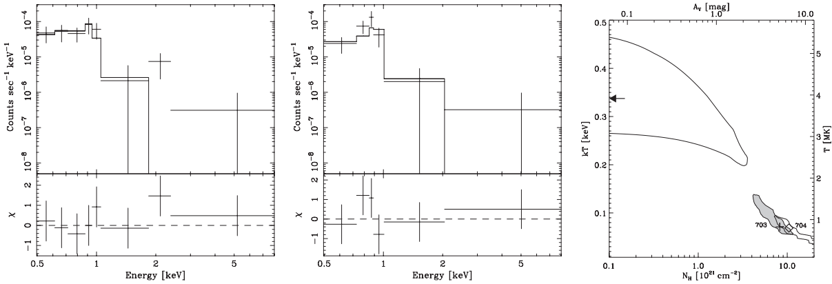
Fig. 3. X-ray spectra of COUP 703 ( left ) and COUP 704 ( middle ), and confidence regions of the plasma parameters ( right ). Each spectral bin contains at least 5 events. We used for the spectral fitting a collisionally-ionized plasma model (APEC), assuming a plasma with solar elemental abundances (Anders & Grevesse 1989), with X-ray absorption model (WABS; Morrison & McCammon 1983). Fit parameters are given in Table 1. In the right panel, the grey region indicates for COUP 703 the confidence region at the 68% level of the plasma temperature and the absorption. The plus sign and diamond mark the best parameter values for COUP 703 and COUP 704 (high N_{\text{H}} /low kT solution), respectively. The arrow indicates the high temperature value for the null absorption solution of COUP 704.
