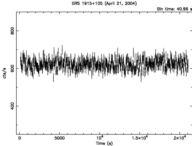
Fig. 2. The source light curve in the 0.4–10.0 keV band during OBS2 (EPIC-pn, burst mode, not background-subtracted). The whole 20 946 s observation has a mean 618 (i.e. 18.54/0.03) cts/s; the background has just about 18 (i.e. 0.5320/0.03) cts/s.
