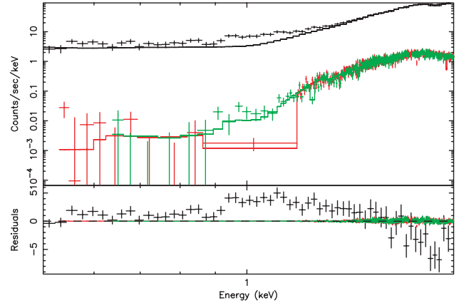
Fig. 4. The RGS and pn (burst mode) spectra fitted in the 0.5–2 keV range with a simple absorbed power law. The RGS and pn spectra clearly disagree each other.
