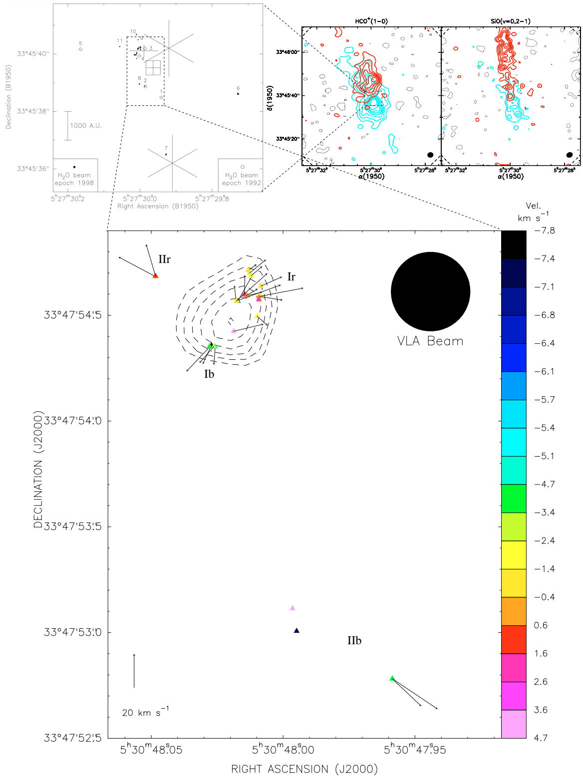
Fig. 3. VLA and VLBA results towards AFGL 5142. Upper right-hand panel: contour maps of the OVRO high-velocity emission of HCO + (1 → 0) ( left ) and SiO ( v = 0, 2 \rightarrow 1 ) ( right ) (Hunter et al. 1999). Upper left-hand panel: positions of the 22 GHz masers detected with the VLA in 1992 ( open squares ) and 1998 ( filled dots ); OVRO 88 GHz ( boxed cross ) and VLA 8.4 GHz ( plain cross ) continuum sources (Hunter et al. 1995, 1999). Bottom panel: positions of the VLBA H 2 O maser features are marked with filled triangles , different colours denote the features' LSR velocities, according to the colour scale on the right-hand side of the panel, and the arrows indicate the measured absolute proper motions, whose amplitude scale is given at the bottom of the panel; the labels Ib, Ir and IIb, IIr individuate the blue-shifted and red-shifted maser clusters of Group I and Group II, respectively; the contour map (with contours representing 5, 6, 7, 8, and 9 times the 50 \mu Jy beam -1 rms noise) shows the 22 GHz VLA continuum emission; the filled circle in the upper right corner represents the restoring beam of the VLA-B 22 GHz continuum map.
