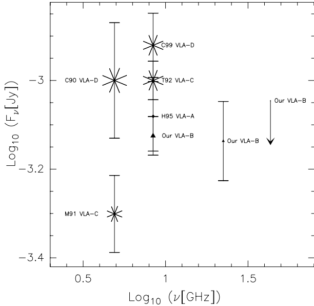
Fig. 2. The radio spectral energy distribution of AFGL 5142. Filled triangles are our VLA-B measurements of the flux density at 8.4 (0.75 mJy with a \approx 0''.9 beam), 22.4 (0.7 mJy with a \approx 0''.4 beam), and 43.3 GHz ( \leq 0.9 mJy with a \approx 0''.2 beam; the upper limit is indicated by the downward arrow). The asterisks are previous flux density measurements at 4.9 GHz (1.0 mJy with a \approx 12''.5 beam using VLA-D – Carpenter et al. 1990 (C90) – and 0.5 mJy with a \approx 4'' beam using VLA-C – McCutcheon et al. 1991 (M91)) and 8.4 GHz (0.83 mJy with a \approx 0''.3 beam using VLA-A – Hunter et al. 1995 (H95); 1.0 mJy with a \approx 7''.7 beam using VLA-C – Torrelles et al. 1992 (T92); 1.2 mJy with a \approx 7''.5 beam using VLA-D – Carral et al. 1999 (C99)). The size of the symbols scales logarithmically with the FWHM size of the beam.
