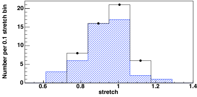
Fig. 7. The stretch ( s parameter) distributions of nearby (hashed blue) and distant (thick black with filled symbols) SNLS SNe with z < 0.8 . These distributions are very similar with averages of 0.920 \pm 0.018 and 0.945 \pm 0.013 , respectively ( 1\sigma apart).
