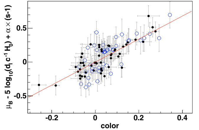
Fig. 10. Residuals in the Hubble diagram as a function of color ( c parameter), for nearby (blue open symbols) and distant ( z < 0.8 , black filled symbols). This diagram computes distance modulus \mu_B without the color term \beta c , and returns the brighter-bluer relationship with a consistent behavior for nearby and distant SNe Ia. Notice that the bluest SNLS objects are compatible with the bulk behavior.
