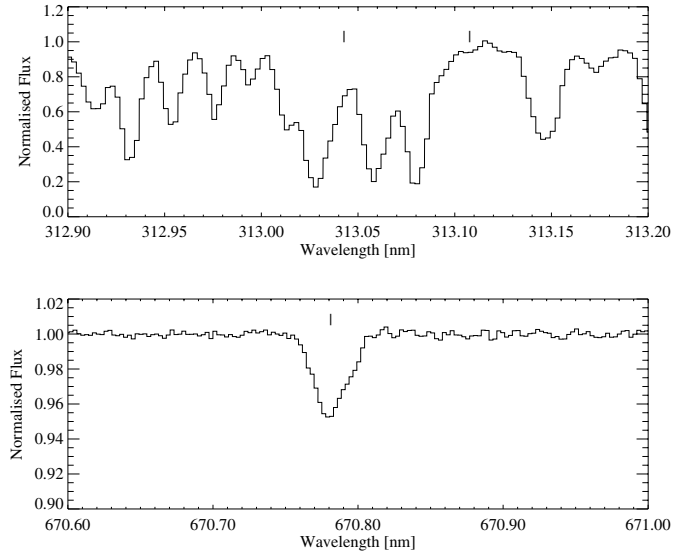
Fig. 1. Spectra of the Be (top) and Li (bottom) regions in one star of our sample, HD 18857. The positions of the Be II doublet and of the Li I line are indicated by vertical bars in both panels.
