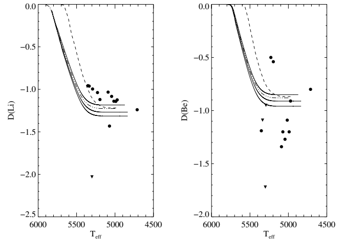
Fig. 5. Observed logarithmic depletion factors (circles) and predictions based on: evolutionary tracks with [\text{Fe}/\text{H}] = -2.27 and stellar masses of 0.75, 0.80 and 0.85 M_{\odot} (solid lines, from top to bottom) from Charbonnel (priv. comm.) and evolutionary track with [\text{Fe}/\text{H}] = -2.30 and stellar mass of 0.775 M_{\odot} (dashed line) from Deliyannis. For comparison, an interpolated model from Charbonnel for a stellar mass of 0.775 M_{\odot} is also presented (dot-dashed line).
