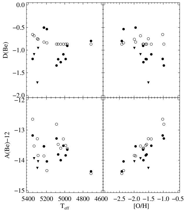
Fig. 8. Logarithmic Be depletion factors ( top panels ) and Be abundances ( bottom panels ) as a function of effective temperature ( left panels ) and oxygen abundance ( right panels ). Our estimates (filled circles) are compared with the predictions (open circles). Stars with upper limits on Be abundance are denoted by triangles.
