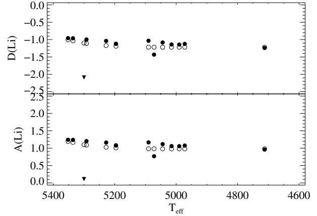
Fig. 4. Logarithmic Li depletion factors ( top panel ) and Li abundances ( bottom panel ) as a function of effective temperature. Observed depletion factors and the NLTE Li abundances (filled circles) on which these factors are based are plotted together with the predicted values (open circles). A value of 2.2 was taken as representative of initial Li abundance. The triangle denotes the star HD 108317 with an upper limit on the Li abundance.
