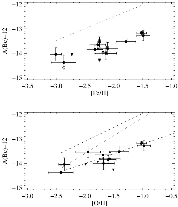
Fig. 6. NLTE and LTE Be abundances as a function of metallicity ( top panel ) and only NLTE values as a function of oxygen abundances ( bottom panel ). The dotted lines correspond to: the Be-vs.-Fe ( top panel ) and the Be-vs.-O ( bottom panel ) correlation for dwarfs from Boesgaard et al. (1999). The dashed lines correspond to the Be-vs.-O correlation for dwarfs from Primas et al. (2005, in preparation, upper line in bottom panel) and for our observed subgiants (lower line in bottom panel).
