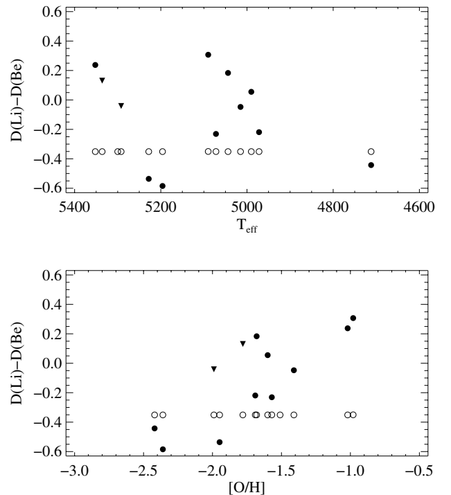
Fig. 9. The differences between logarithmic depletion factors for Li and Be as a function of temperature ( top panel ) and oxygen abundance ( bottom panel ). Estimates (filled circles) are compared with predictions based on Deliyannis et al. (1990) (open circles).
