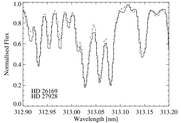
Fig. 7. The UV Be II doublet lines in the observed spectra of HD 26169 (solid line) and HD 27928 (dot-dashed line).
