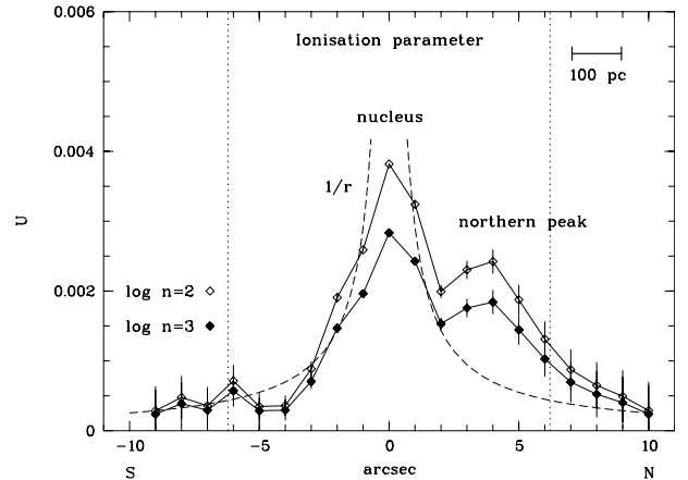
Fig. 11. Ionisation parameter derived from [O II]/[O III] ratio as a function of distance from the nucleus (open symbols: n_H = 100 \text{ cm}^{-3} , filled ones: n_H = 1000 \text{ cm}^{-3} ). The ionisation parameter is highest in the center and decreases with distance with a secondary peak at 4'' to the north of the center. The fit U(r) = U_0 r^{-1} is shown as dashed line. The edge of the NLR as determined from the diagnostic diagrams is indicated by dotted lines.
