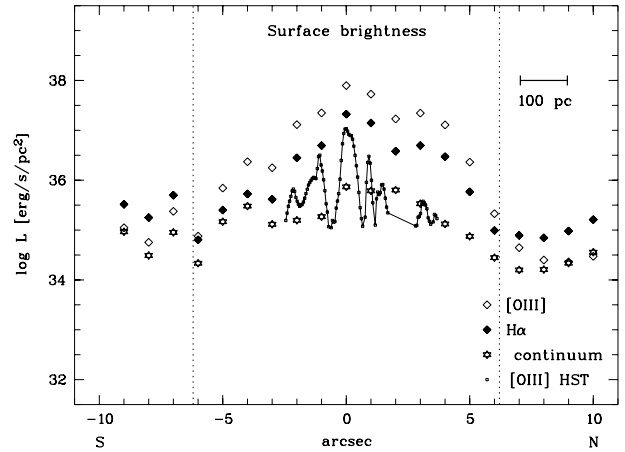
Fig. 9. Surface-brightness distribution of NGC 1386 in [O III] (open diamonds), H \alpha (filled diamonds), and continuum (at 5450–5700 Å, stars). Error bars are smaller than the symbol size. The [O III] surface-brightness distribution from the HST image with S/N > 3 is shown as small open squares connected by a line. The HST image has a 20 times higher spatial resolution but a significantly lower sensitivity, not allowing to measure the outer parts of the NLR. The edge of the NLR as determined from the diagnostic diagrams is indicated by dotted lines.
