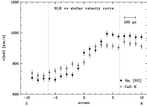
Fig. 12. Velocity curve of the NLR derived from the average value of the peak wavelengths of the H\alpha and [N\text{II}] emission lines (filled symbols) as well as the stellar velocity curve measured using the Ca II K absorption-line “peak” wavelength as seen in the “raw” spectrum (open symbols). The edge of the NLR as determined from the diagnostic diagrams is indicated by dotted lines.
