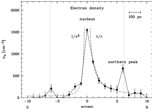
Fig. 10. Electron density obtained from the [S II] \lambda 6716 \text{ \AA}/\lambda 6731 \text{ \AA} ratio as a function of distance from the nucleus. Open symbols indicate locations where n_e is in the low-density limit (assumed \leq 50 \text{ cm}^{-3} ). The electron density decreases with radius and shows a secondary peak 6'' north of the nucleus as well as a tertiary fainter one at 6'' south. The fits n_e(r) = n_{e,0} r^{-1} and n_e(r) = n_{e,0} r^{-2} are shown as dashed lines. The edge of the NLR as determined from the diagnostic diagrams is indicated by dotted lines.
