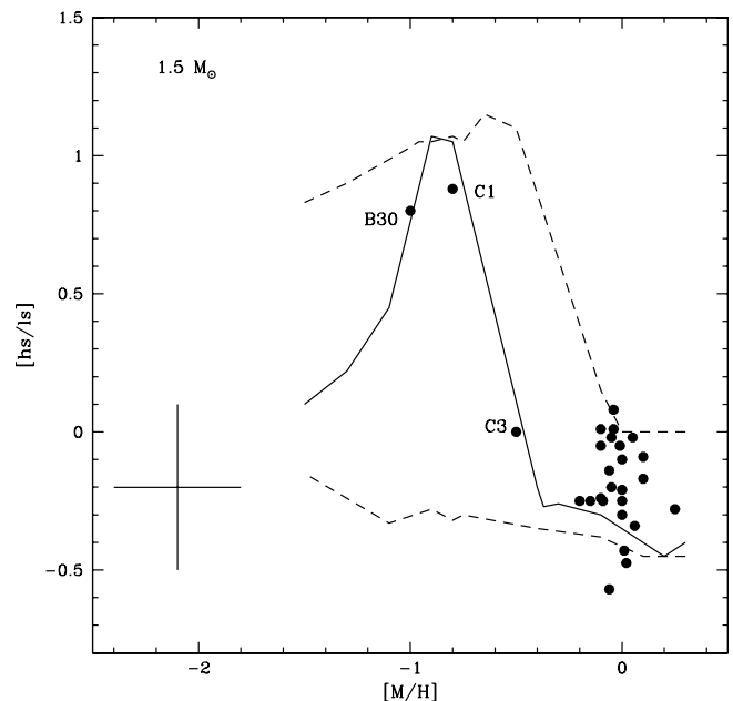
Fig. 6. Comparison of the observed mean of heavy (Ba, La, Nd and Sm) to light-mass (Sr, Y and Zr) s-element [\text{hs}/\text{ls}] enhancement (signature of the neutron exposure) against metallicity with theoretical prediction for a 1.5 M_{\odot} TP-AGB. Continuous and dashed lines represent the same as Fig. 5. The location of the stars studied here are marked. At near solar metallicity, the galactic carbon stars studied in Abia et al. (2002, after minor revisions) are shown for comparison.
