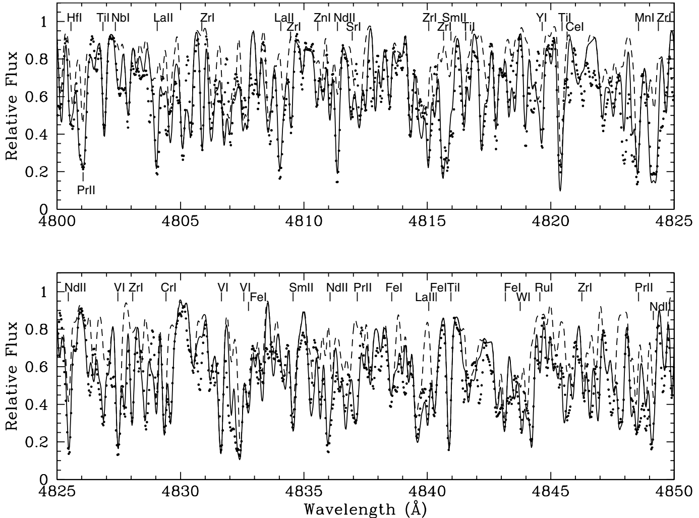
Fig. 2. Synthetic fits to the spectrum of the star IGI95-C1 in the region around 4825 Å. From this region we derived most of the s-elements abundances and the mean metallicity of the stars. Some atomic lines, main contributors to the specific spectral feature, are marked. Black dots represent the observed spectrum. Lines are synthetic spectra: only molecules and metals (dashed line), and including s-elements (best fit, continuous line).
