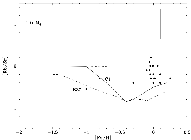
Fig. 5. Comparison of the observed [\text{Rb}/\text{Sr}] ratio vs. [\text{M}/\text{H}] with the theoretical predictions for different choices of the ^{13}\text{C} -pocket (see text) for a 1.5 M_{\odot} TP-AGB. Continuous line represents the ST (standard) choice while dashed lines limit the area allowed by the choices from \text{ST}\times 2 to \text{ST}/12 . Theoretical models are from Gallino et al. (1998). The stars studied here are marked. The abundance ratios corresponding to IGI95-C3 are not shown because we do not detected Rb in this star. Similar ratios derived in galactic N-type carbon stars (Abia et al. 2001) (black dots at near solar metallicity) are also shown for comparison.
