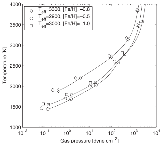
Fig. 1. Temperature structures of the model atmospheres computed with the stellar parameters corresponding to the three stars studied in this work. The points where the optical depth \log \tau_{\text{Ross}} = -4, -3, \dots, 0 are indicated by markers. The models corresponding to IGI95-C1 are marked with diamonds, IGI95-C3 with circles and BMB-B 30 with squares. The structure is very sensitive to the carbon excess. The structures computed with the lower value of C/O in Table 3 are plotted with solid lines and markers while the structures with high C/O are indicated with markers only.
