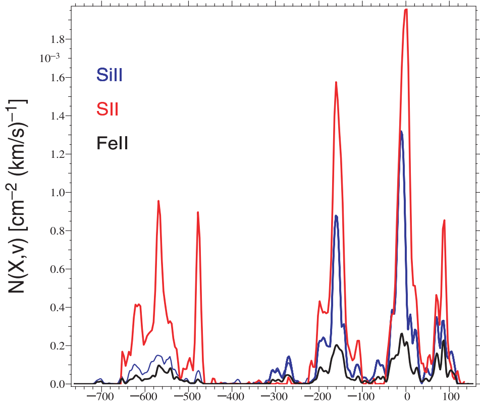
Fig. 7. This panel shows the optical depth profiles in the z_{\text{abs}} = 1.973 DLA toward Q 0013–004. The apparent column density per velocity bin -N(X, dv) ( y axis values are scaled to \times 10^{-3} ) – is represented on a velocity scale, with v = 0 \text{ km s}^{-1} centered at z_{\text{abs}} = 1.973 .
