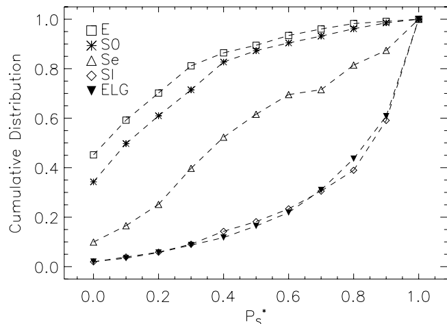
Fig. 5. The normalized cumulative P_{S^*} -distributions of the 4 morphological galaxy classes and of the emission-line galaxies.
