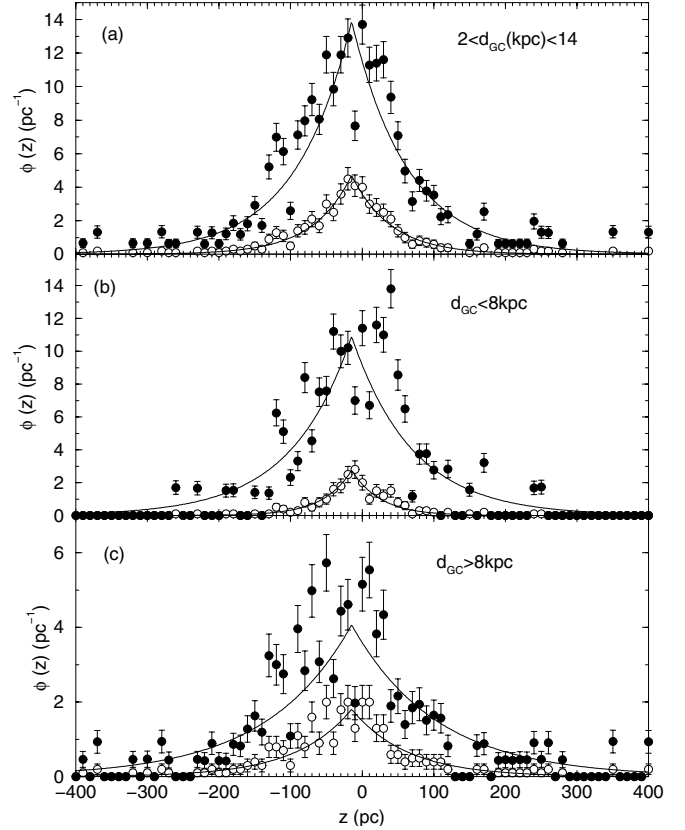
Fig. 15. Completeness-corrected z -distributions. Panel a ): overall radial distribution (scale height z_h \approx 78 pc). Panel b ): OCs internal to the Solar circle ( z_h \approx 85 pc). Panel c ): OCs external to the Solar circle ( z_h \approx 119 pc). Empty circles: observed OCs. Filled circles: completeness-corrected z -distribution.
