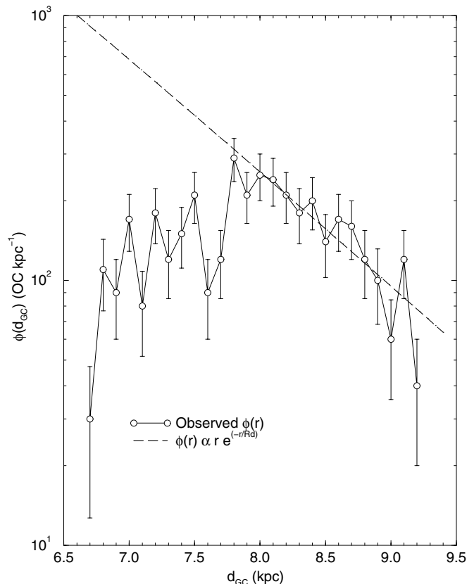
Fig. 9. Observed distribution function of OCs in terms of Galactocentric distance in the restricted zone. Dashed line: exponential-disk distribution \phi(r) \propto r e^{-(r/R_D)} . Note the depletion in the number of OCs for d_{\text{GC}} \leq 7.8 kpc, and the V-shaped dip at d_{\text{GC}} \approx 7.5\text{--}7.8 kpc.
