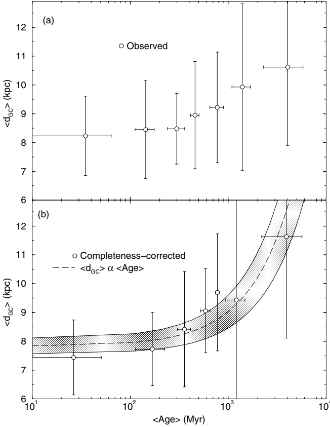
Fig. 17. Relation of Galactocentric distance and age. Panel a ): observed OCs. Panel b ): completeness-corrected. The bars show the 1 \sigma -standard deviations of the average values of age and Galactocentric distance within the respective bins. Dashed line: linear-least squares fit to the completeness-corrected points. Shaded region: 1 \sigma -standard deviation of the fit.
