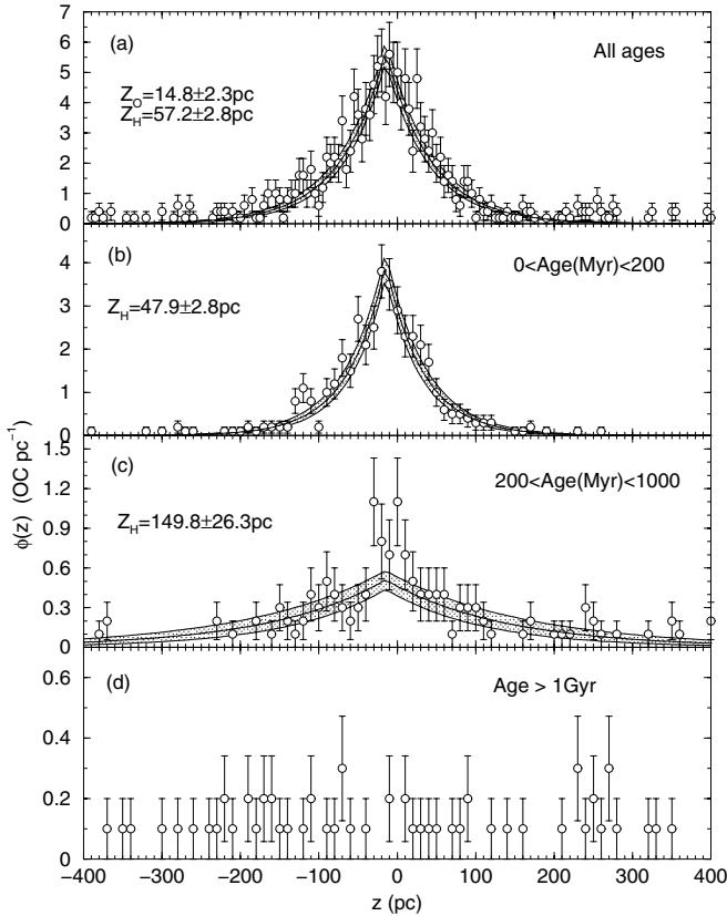
Fig. 7. Distribution of OCs in terms of height over the Galactic plane. Age groups are considered separately. Solid lines: least-squares fit with \phi(z) = \phi_0 e^{-|(z+z_\odot)/z_h|} . Shaded areas: 1\sigma -standard deviation. Top panel: bins of 5 pc in z . Bottom panels: 10 pc bins.
